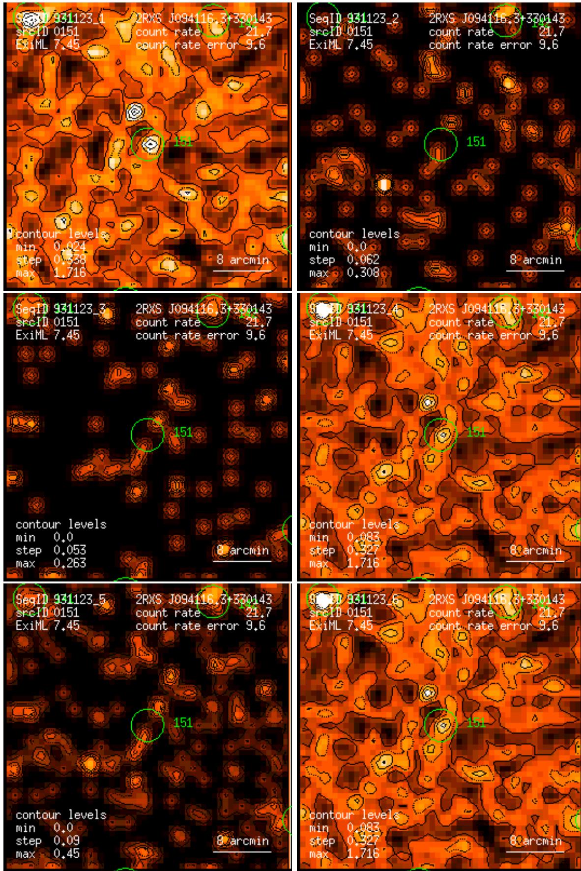
Figure 151: RASS 931123: detection 0151: band rate images, Gaussian filter: (1) PSPC channels 11 – 41, (2) 52 – 90, (3) 91 – 201, (4) 11 – 235, (5) 52 – 201, (6) 11 – 201. Broad band rates in counts/ks. Band rate contour levels in counts/ks/arcmin 2 .
