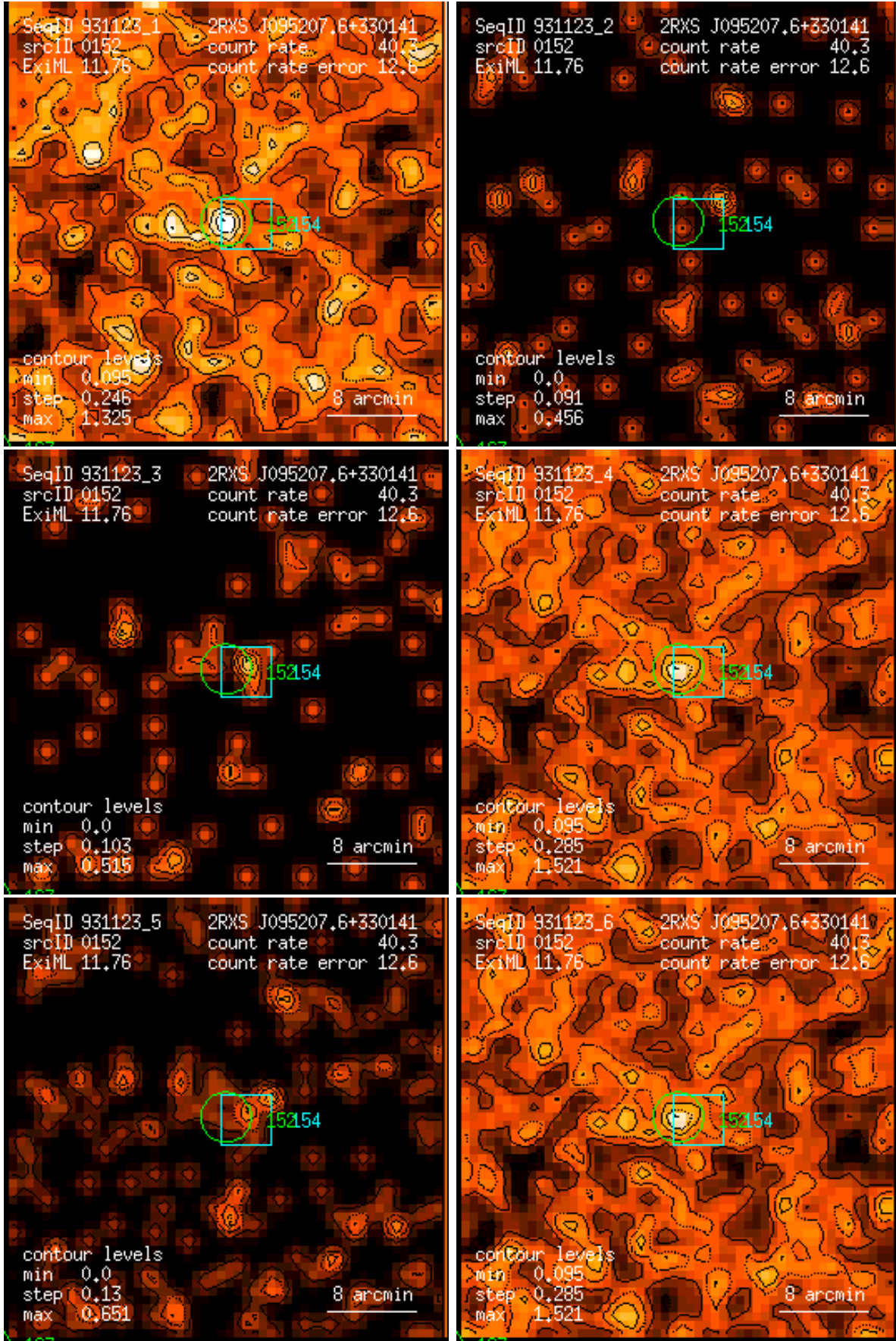
Figure 152: RASS 931123: detection 0152: band rate images, Gaussian filter: (1) PSPC channels 11 – 41, (2) 52 – 90, (3) 91 – 201, (4) 11 – 235, (5) 52 – 201, (6) 11 – 201. Broad band rates in counts/ks. Band rate contour levels in counts/ks/arcmin 2 .
