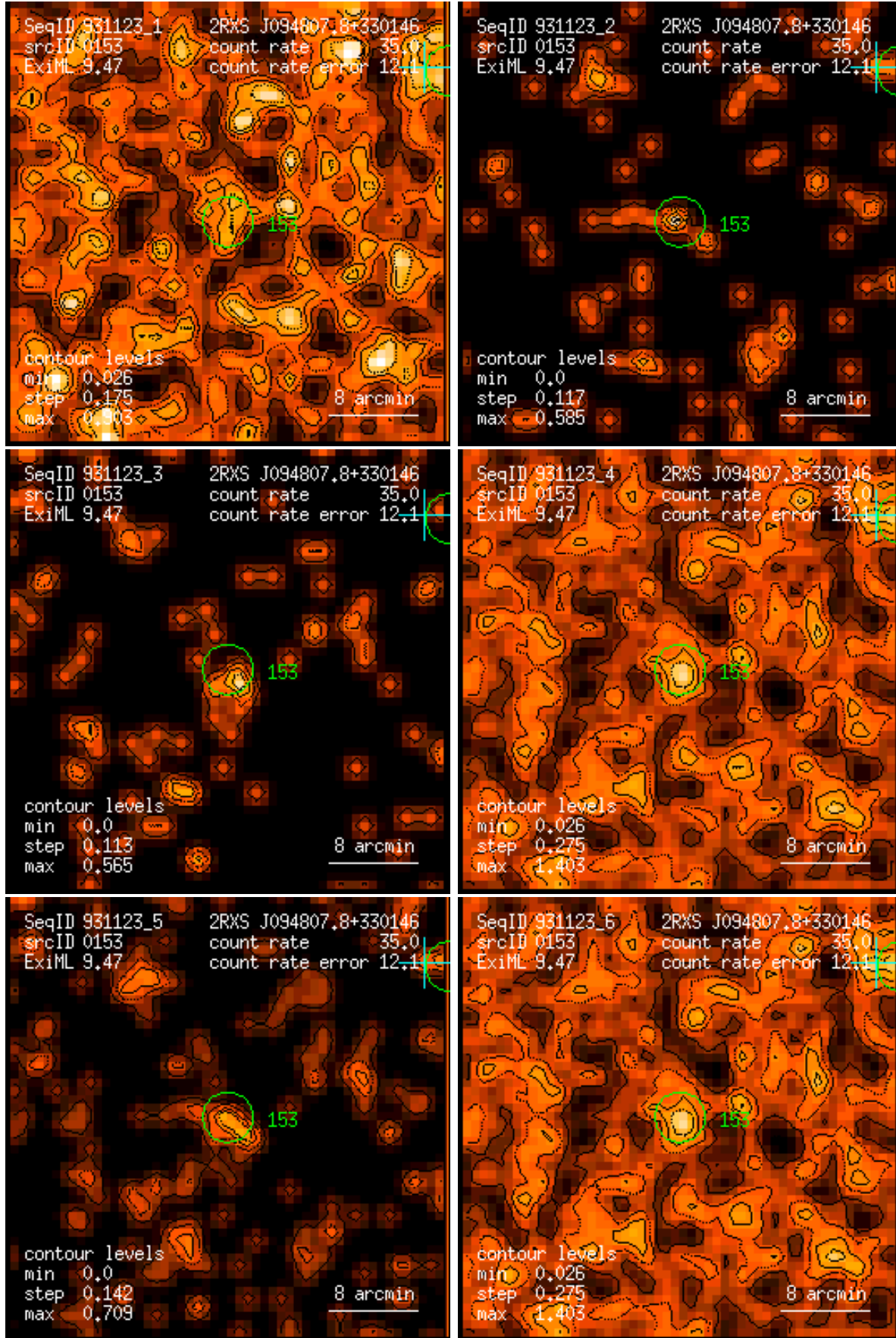
Figure 153: RASS 931123: detection 0153: band rate images, Gaussian filter: (1) PSPC channels 11 – 41, (2) 52 – 90, (3) 91 – 201, (4) 11 – 235, (5) 52 – 201, (6) 11 – 201. Broad band rates in counts/ks. Band rate contour levels in counts/ks/arcmin 2 .
