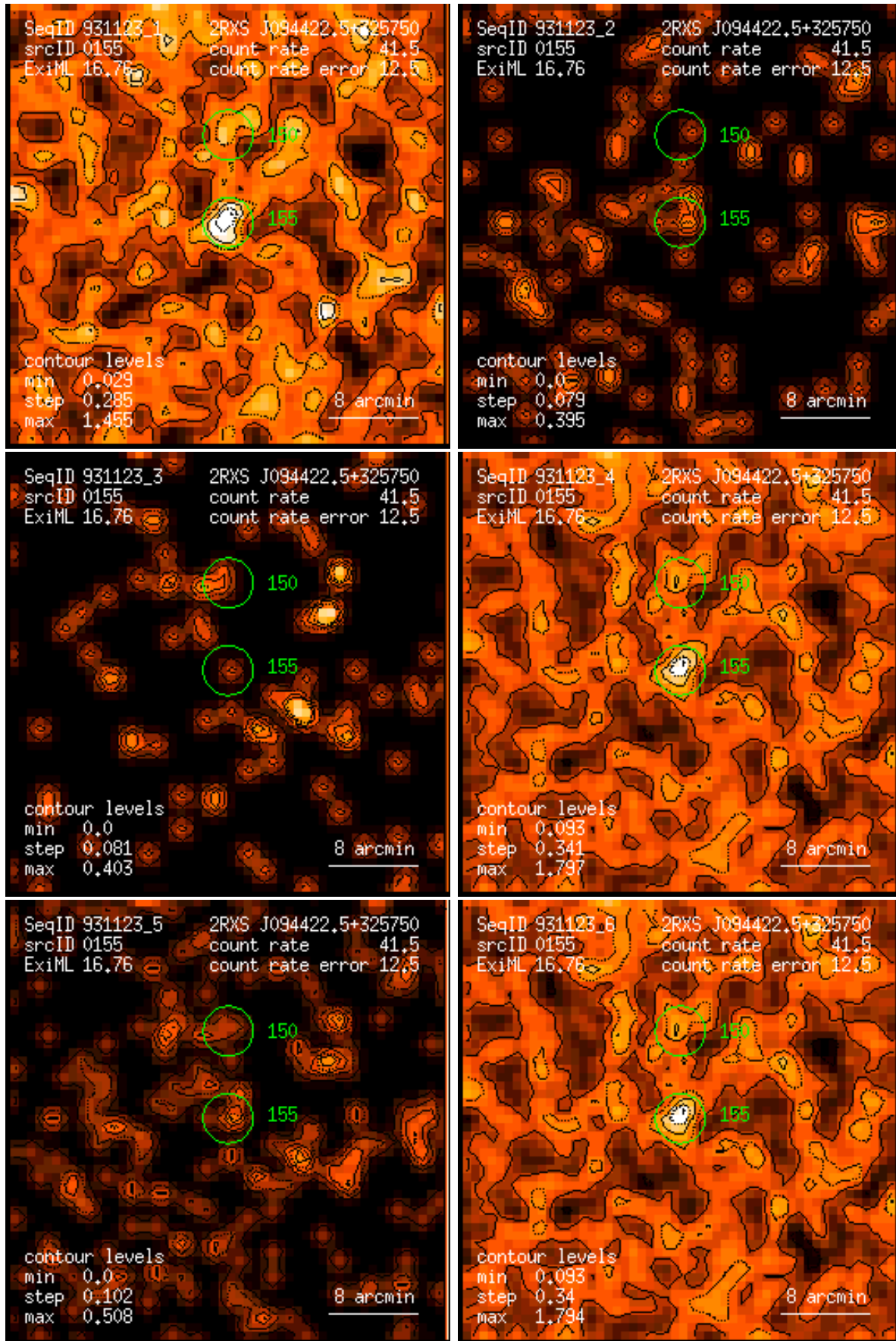
Figure 155: RASS 931123: detection 0155: band rate images, Gaussian filter: (1) PSPC channels 11 – 41, (2) 52 – 90, (3) 91 – 201, (4) 11 – 235, (5) 52 – 201, (6) 11 – 201. Broad band rates in counts/ks. Band rate contour levels in counts/ks/arcmin 2 .
