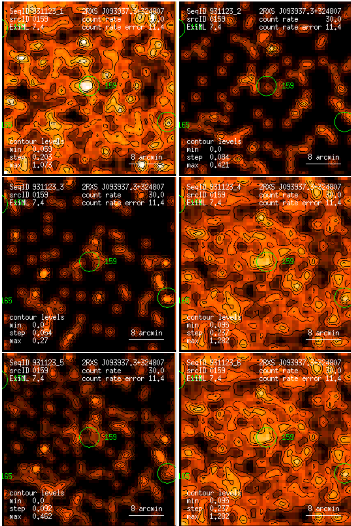
Figure 159: RASS 931123: detection 0159: band rate images, Gaussian filter: (1) PSPC channels 11 – 41, (2) 52 – 90, (3) 91 – 201, (4) 11 – 235, (5) 52 – 201, (6) 11 – 201. Broad band rates in counts/ks. Band rate contour levels in counts/ks/arcmin 2 .
