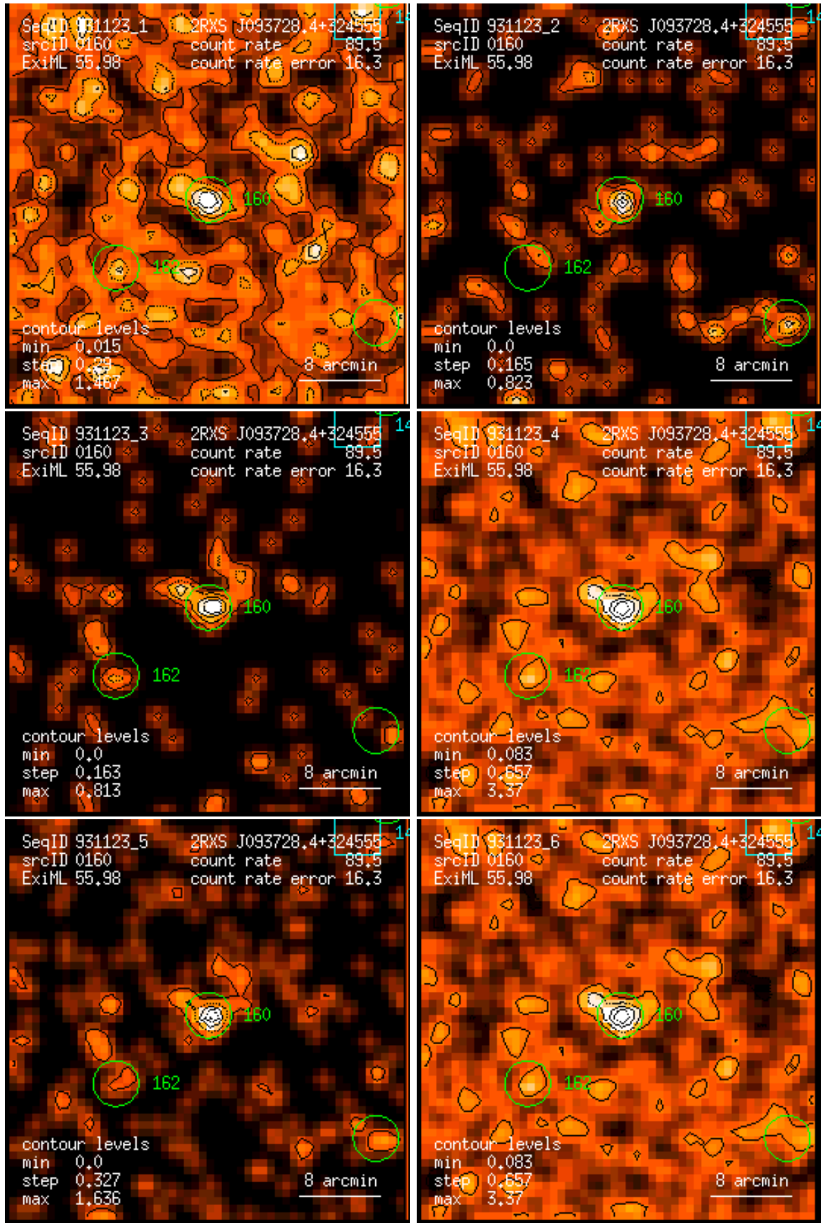
Figure 160: RASS 931123: detection 0160: band rate images, Gaussian filter: (1) PSPC channels 11 – 41, (2) 52 – 90, (3) 91 – 201, (4) 11 – 235, (5) 52 – 201, (6) 11 – 201. Broad band rates in counts/ks. Band rate contour levels in counts/ks/arcmin 2 .
