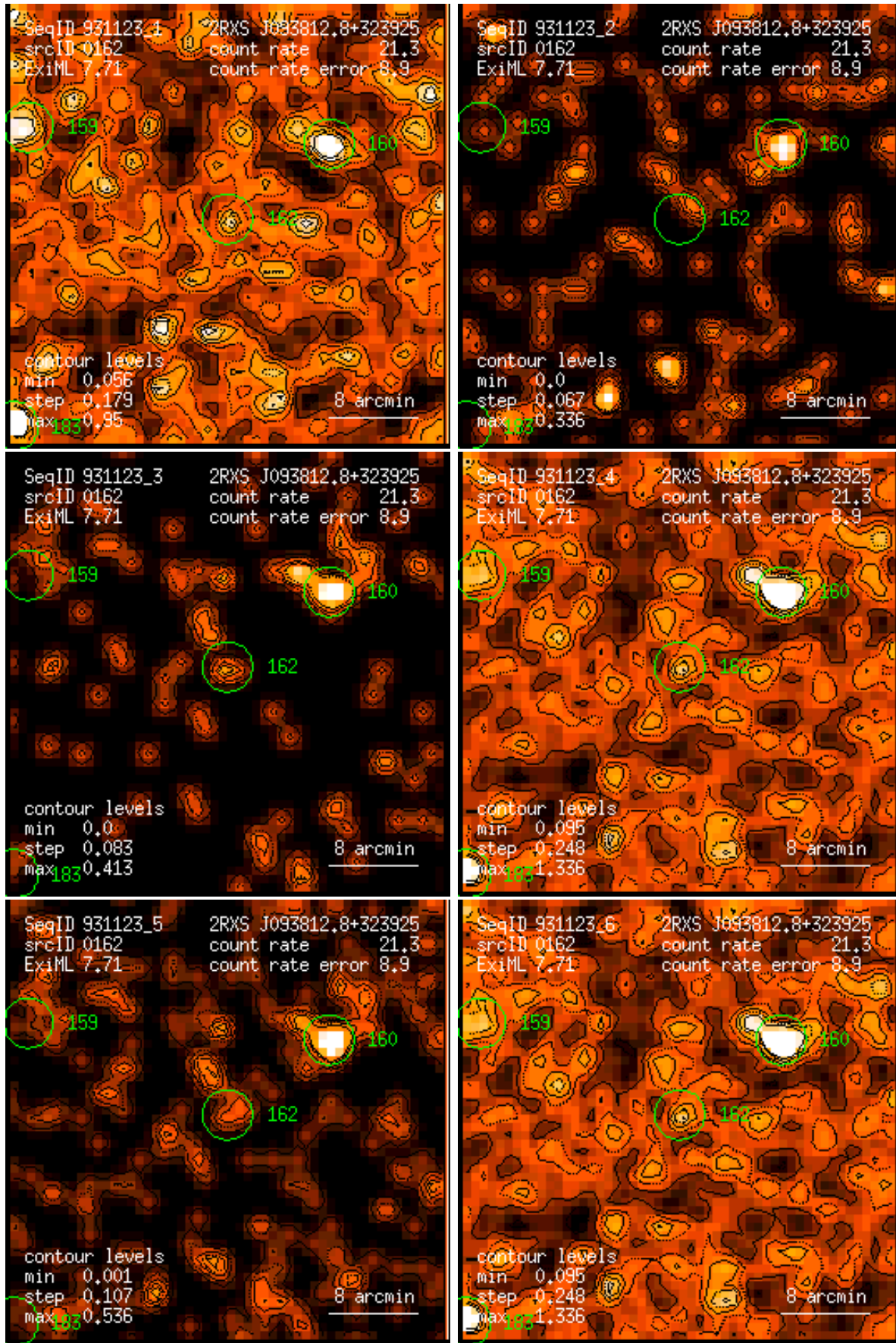
Figure 162: RASS 931123: detection 0162: band rate images, Gaussian filter: (1) PSPC channels 11 – 41, (2) 52 – 90, (3) 91 – 201, (4) 11 – 235, (5) 52 – 201, (6) 11 – 201. Broad band rates in counts/ks. Band rate contour levels in counts/ks/arcmin 2 .
