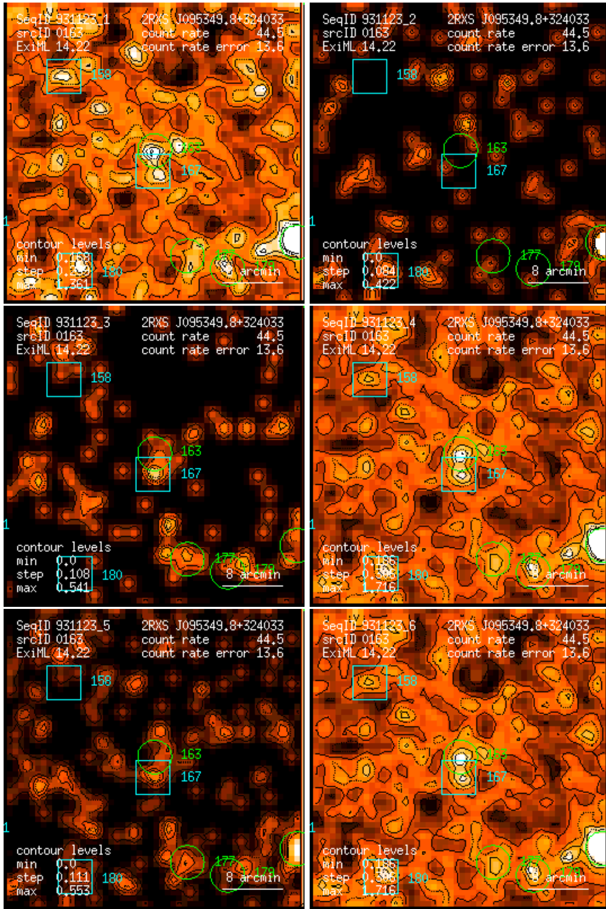
Figure 163: RASS 931123: detection 0163: band rate images, Gaussian filter: (1) PSPC channels 11 – 41, (2) 52 – 90, (3) 91 – 201, (4) 11 – 235, (5) 52 – 201, (6) 11 – 201. Broad band rates in counts/ks. Band rate contour levels in counts/ks/arcmin 2 .
