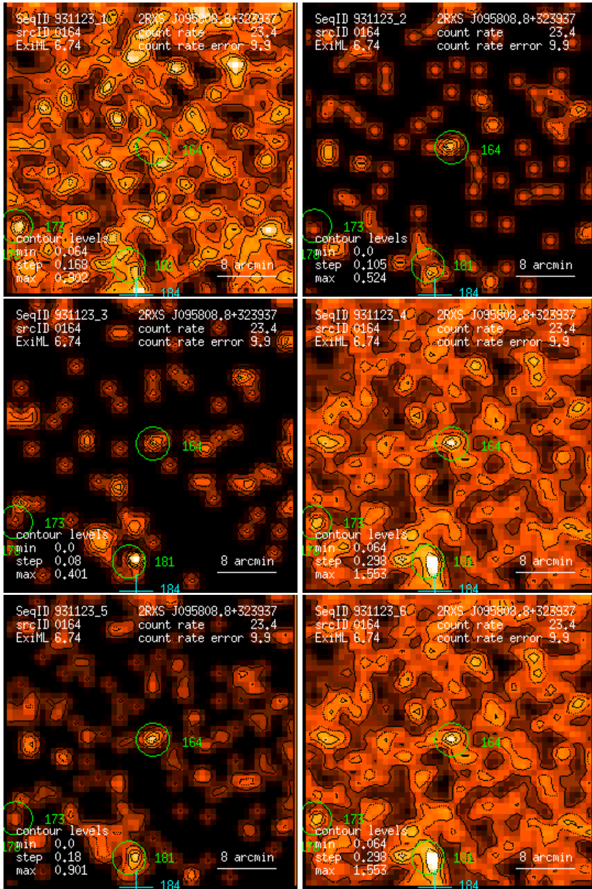
Figure 164: RASS 931123: detection 0164: band rate images, Gaussian filter: (1) PSPC channels 11 – 41, (2) 52 – 90, (3) 91 – 201, (4) 11 – 235, (5) 52 – 201, (6) 11 – 201. Broad band rates in counts/ks. Band rate contour levels in counts/ks/arcmin 2 .
