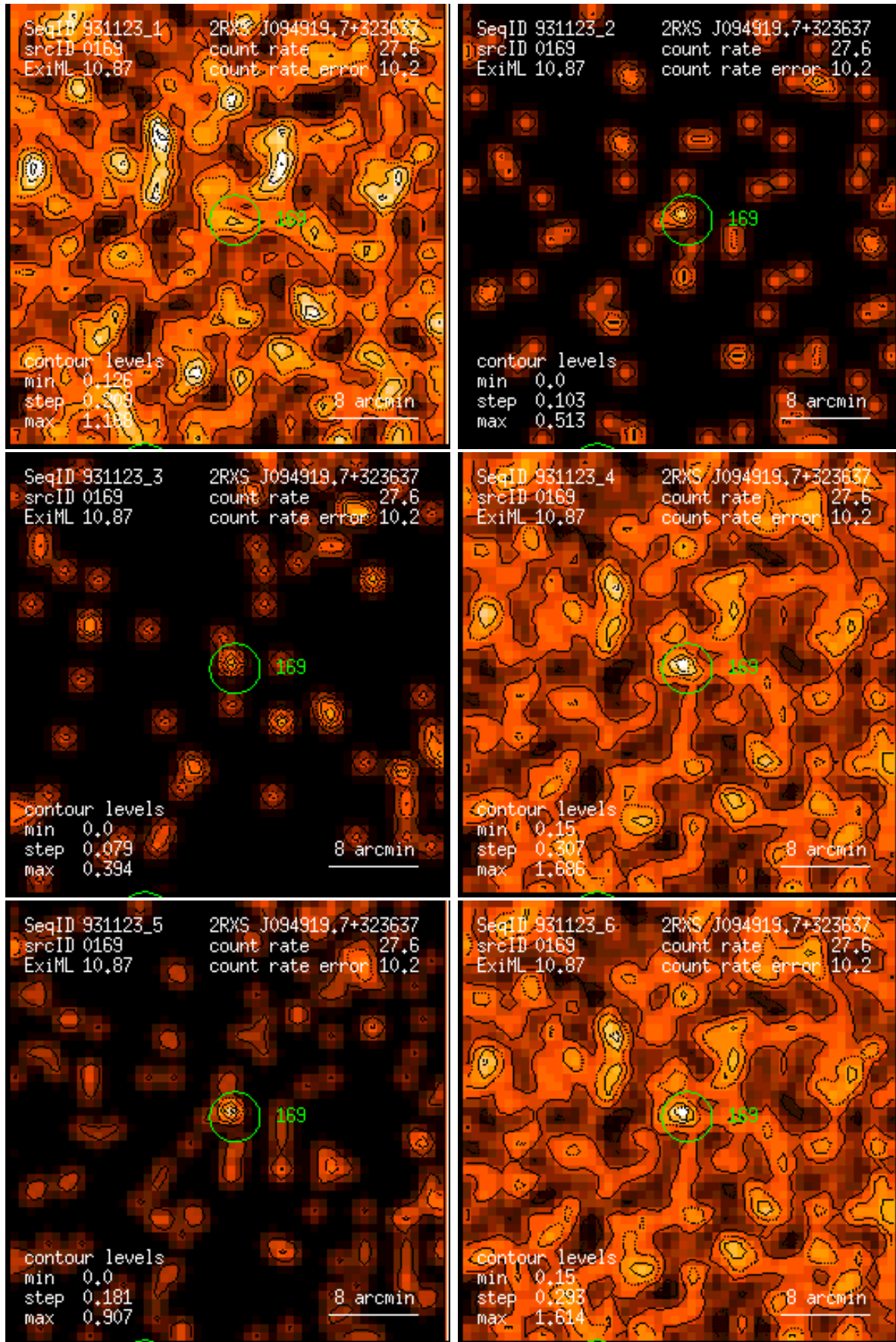
Figure 169: RASS 931123: detection 0169: band rate images, Gaussian filter: (1) PSPC channels 11 – 41, (2) 52 – 90, (3) 91 – 201, (4) 11 – 235, (5) 52 – 201, (6) 11 – 201. Broad band rates in counts/ks. Band rate contour levels in counts/ks/arcmin 2 .
