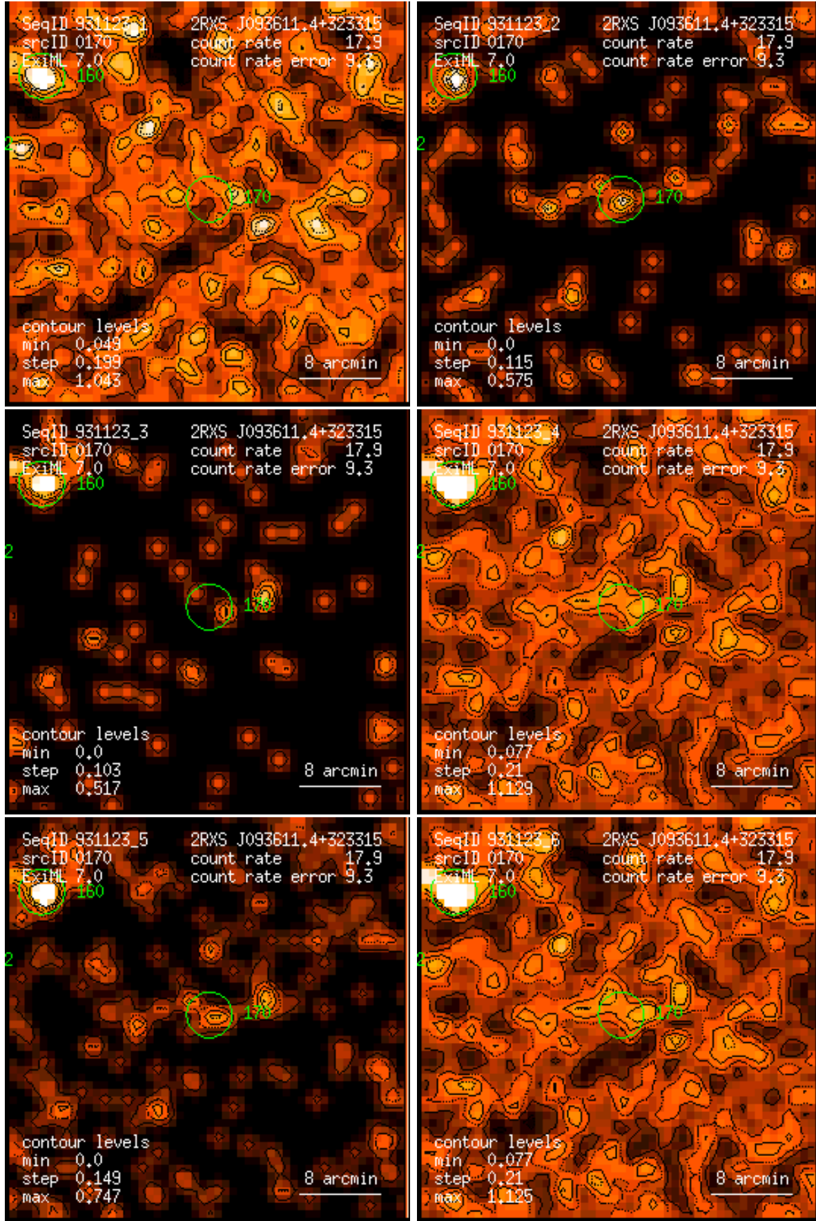
Figure 170: RASS 931123: detection 0170: band rate images, Gaussian filter: (1) PSPC channels 11 – 41, (2) 52 – 90, (3) 91 – 201, (4) 11 – 235, (5) 52 – 201, (6) 11 – 201. Broad band rates in counts/ks. Band rate contour levels in counts/ks/arcmin 2 .
