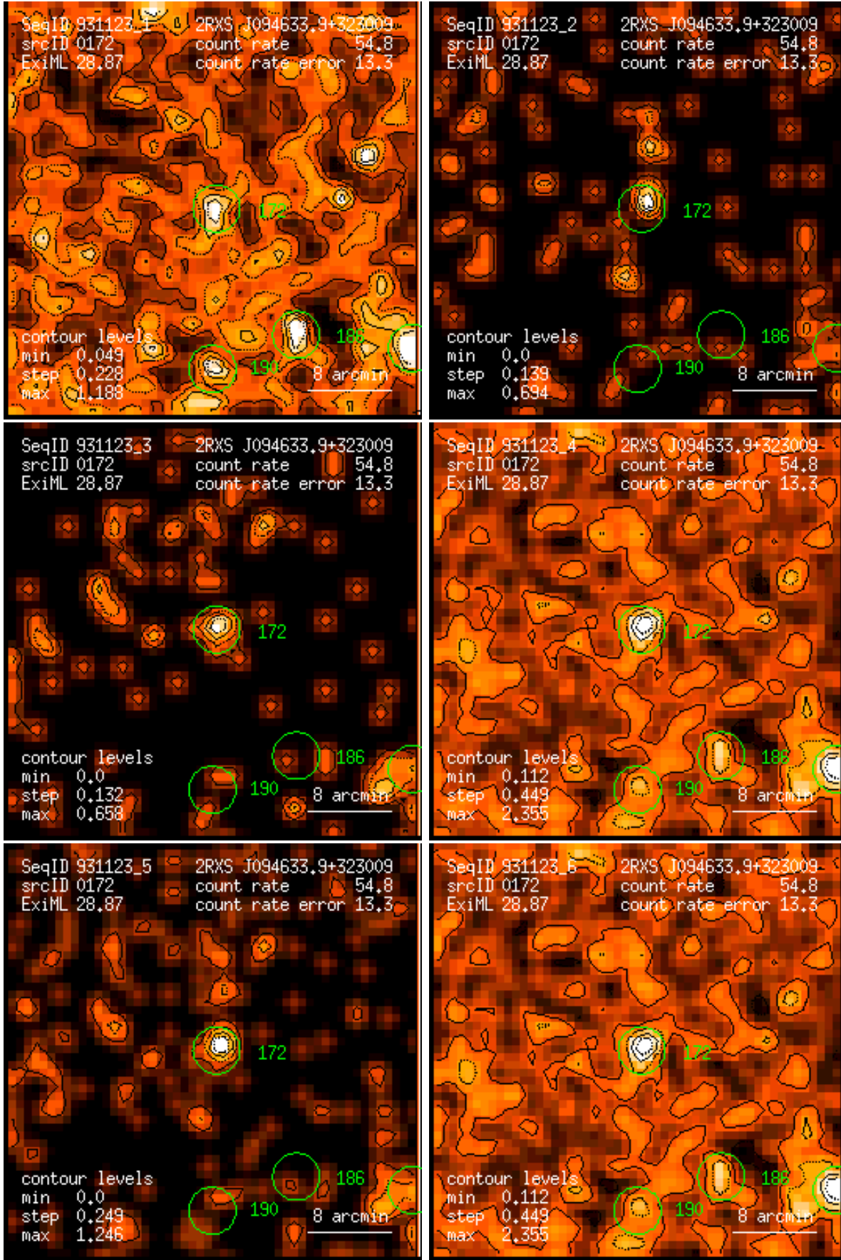
Figure 172: RASS 931123: detection 0172: band rate images, Gaussian filter: (1) PSPC channels 11 – 41, (2) 52 – 90, (3) 91 – 201, (4) 11 – 235, (5) 52 – 201, (6) 11 – 201. Broad band rates in counts/ks. Band rate contour levels in counts/ks/arcmin 2 .
