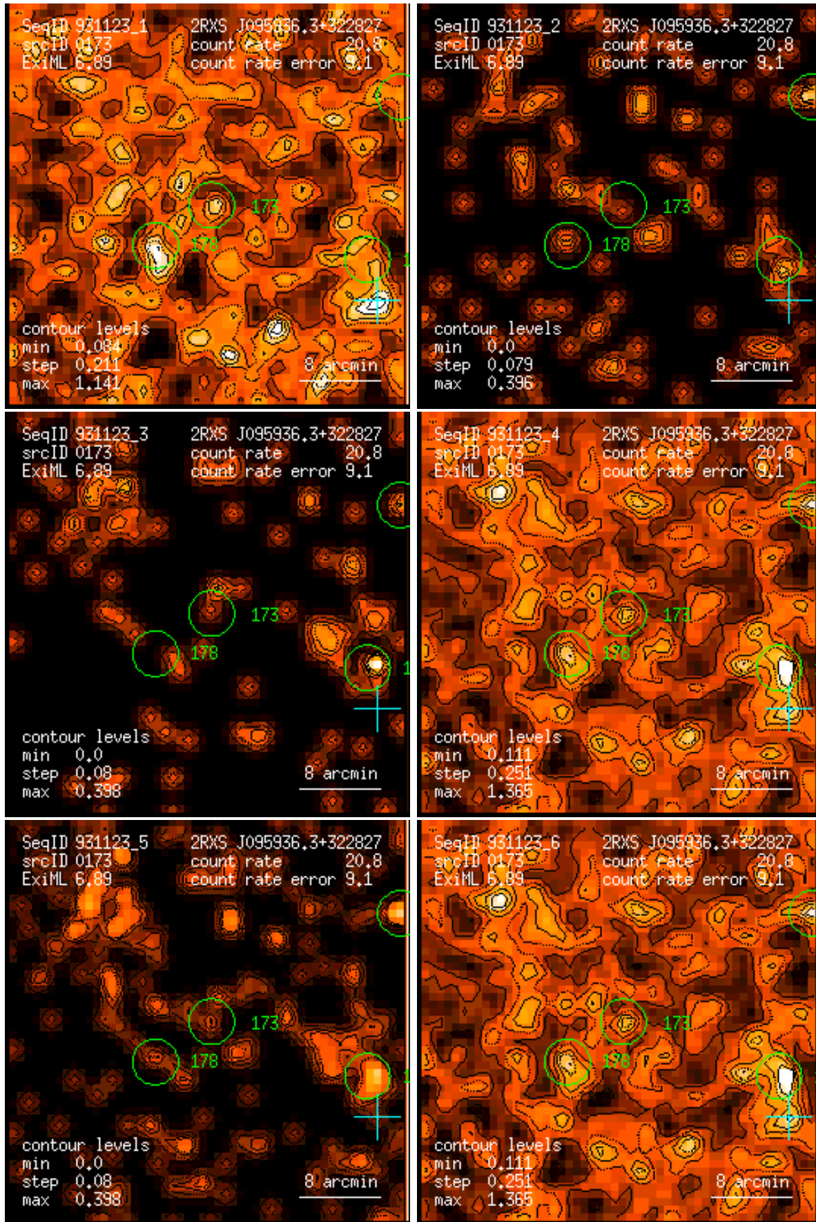
Figure 173: RASS 931123: detection 0173: band rate images, Gaussian filter: (1) PSPC channels 11 – 41, (2) 52 – 90, (3) 91 – 201, (4) 11 – 235, (5) 52 – 201, (6) 11 – 201. Broad band rates in counts/ks. Band rate contour levels in counts/ks/arcmin 2 .
