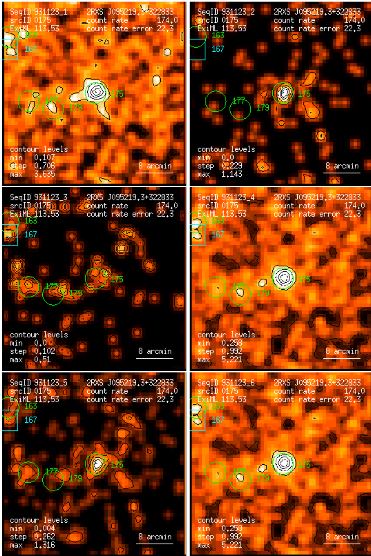
Figure 175: RASS 931123: detection 0175: band rate images, Gaussian filter: (1) PSPC channels 11 – 41, (2) 52 – 90, (3) 91 – 201, (4) 11 – 235, (5) 52 – 201, (6) 11 – 201. Broad band rates in counts/ks. Band rate contour levels in counts/ks/arcmin 2 .
