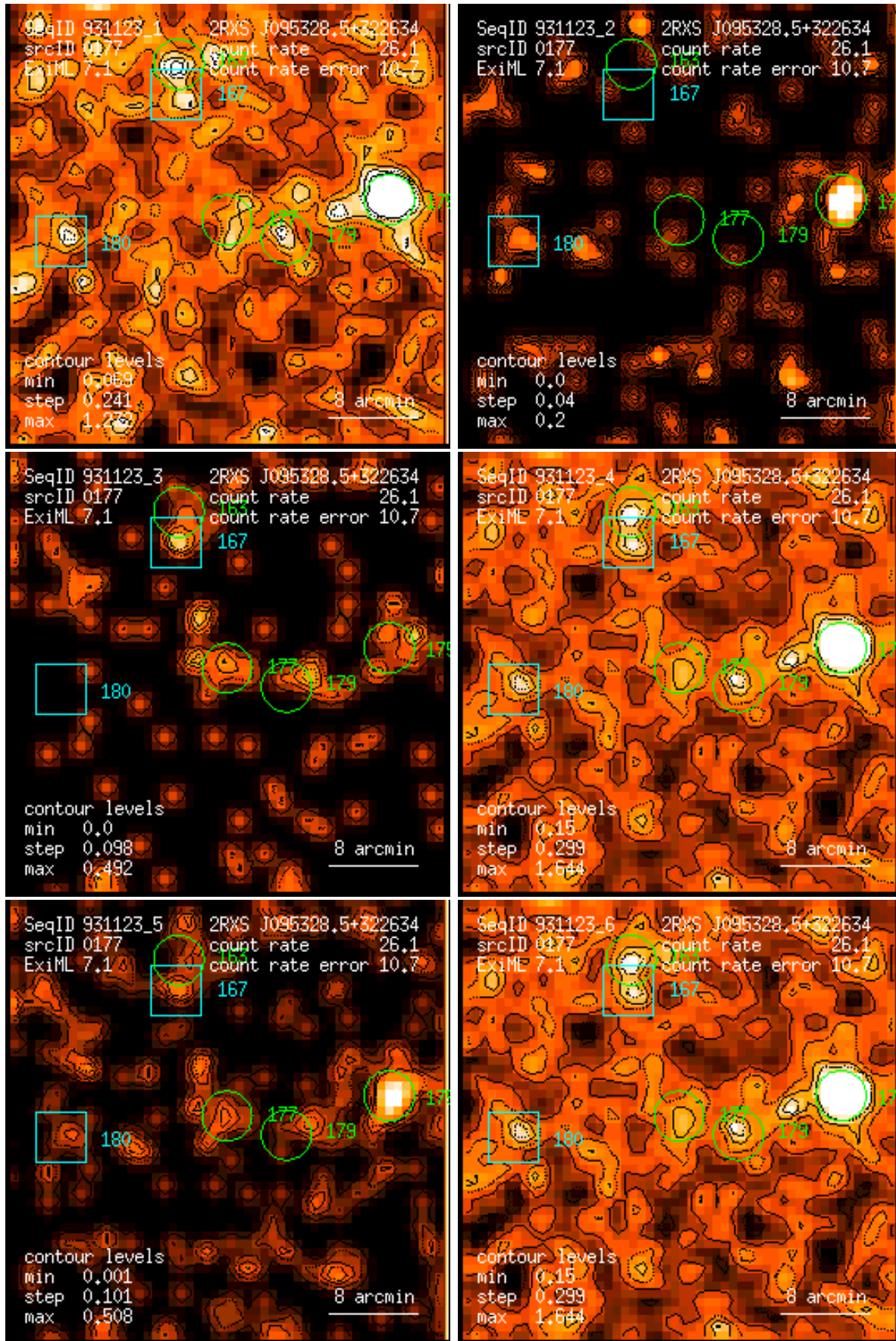
Figure 177: RASS 931123: detection 0177: band rate images, Gaussian filter: (1) PSPC channels 11 – 41, (2) 52 – 90, (3) 91 – 201, (4) 11 – 235, (5) 52 – 201, (6) 11 – 201. Broad band rates in counts/ks. Band rate contour levels in counts/ks/arcmin 2 .
