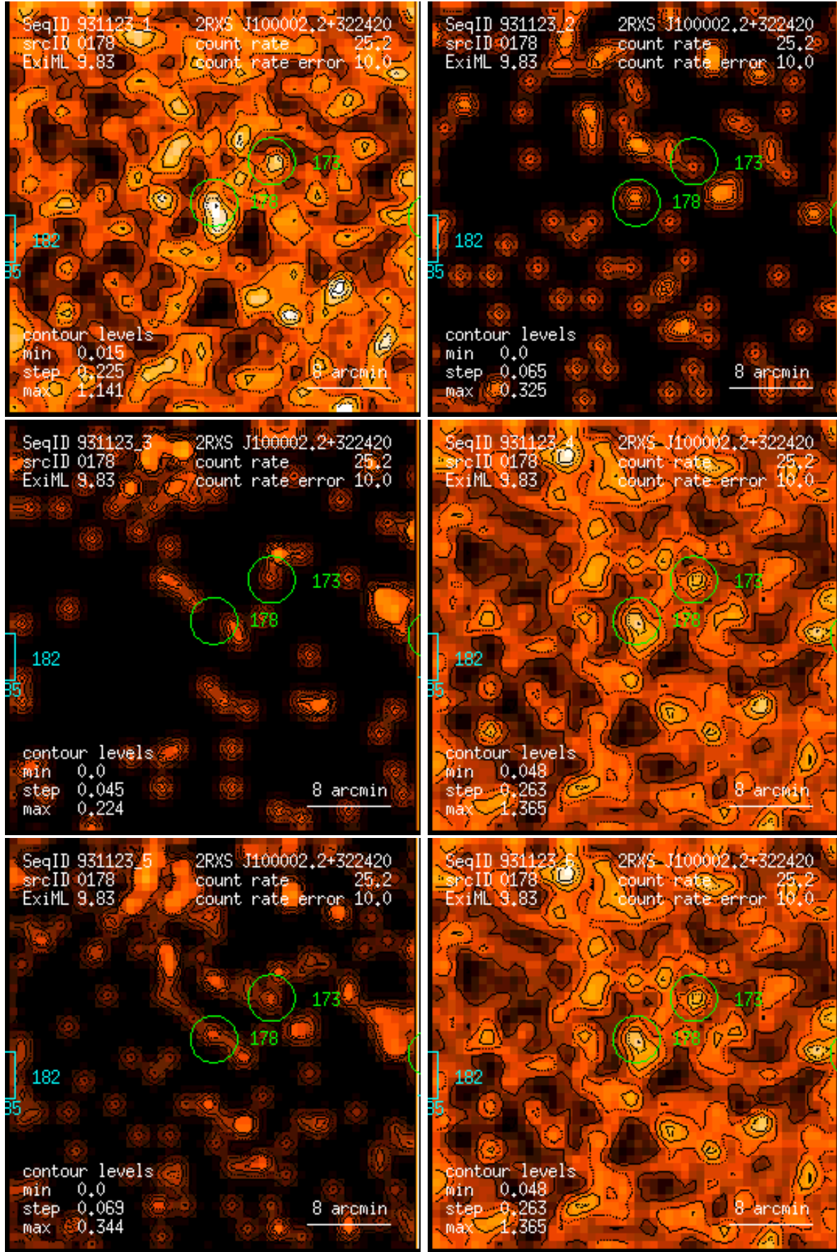
Figure 178: RASS 931123: detection 0178: band rate images, Gaussian filter: (1) PSPC channels 11 – 41, (2) 52 – 90, (3) 91 – 201, (4) 11 – 235, (5) 52 – 201, (6) 11 – 201. Broad band rates in counts/ks. Band rate contour levels in counts/ks/arcmin 2 .
