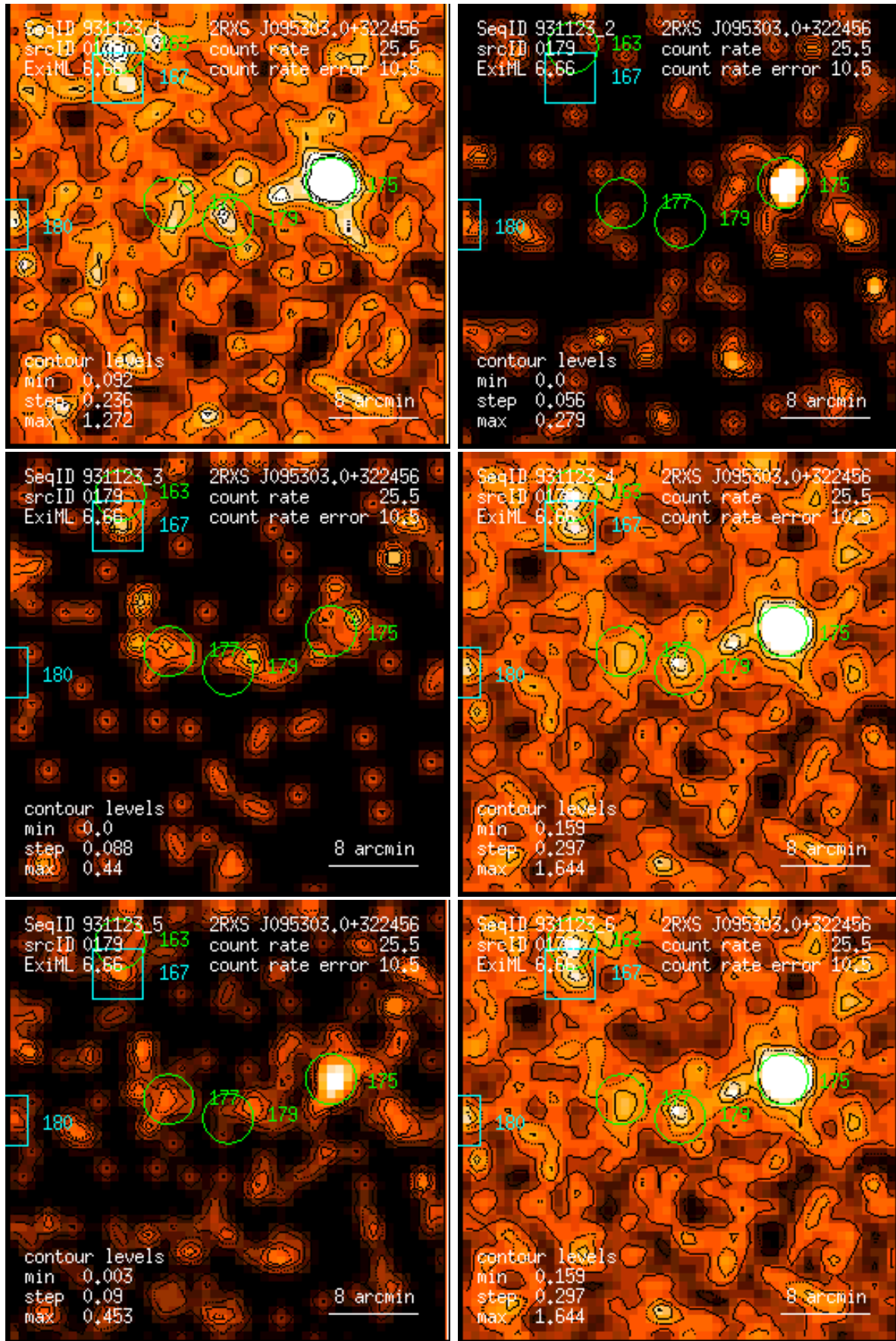
Figure 179: RASS 931123: detection 0179: band rate images, Gaussian filter: (1) PSPC channels 11 – 41, (2) 52 – 90, (3) 91 – 201, (4) 11 – 235, (5) 52 – 201, (6) 11 – 201. Broad band rates in counts/ks. Band rate contour levels in counts/ks/arcmin 2 .
