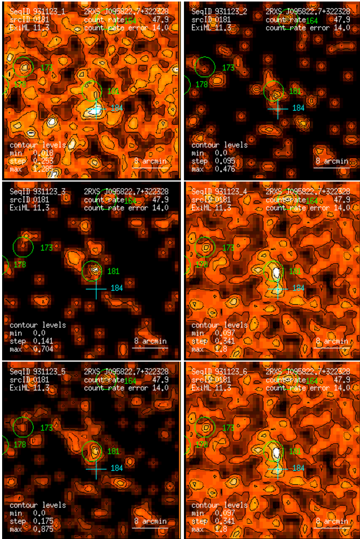
Figure 181: RASS 931123: detection 0181: band rate images, Gaussian filter: (1) PSPC channels 11 – 41, (2) 52 – 90, (3) 91 – 201, (4) 11 – 235, (5) 52 – 201, (6) 11 – 201. Broad band rates in counts/ks. Band rate contour levels in counts/ks/arcmin 2 .
