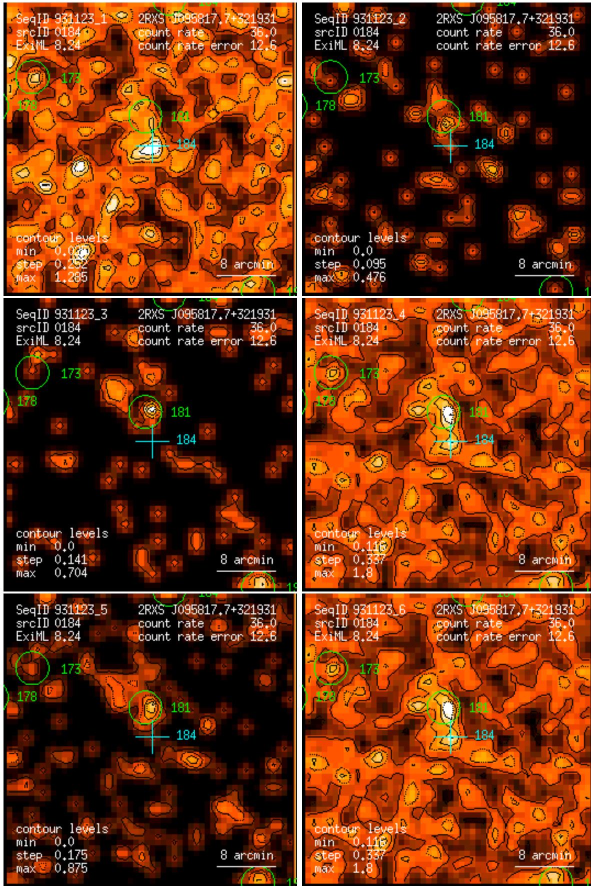
Figure 184: RASS 931123: detection 0184: band rate images, Gaussian filter: (1) PSPC channels 11 – 41, (2) 52 – 90, (3) 91 – 201, (4) 11 – 235, (5) 52 – 201, (6) 11 – 201. Broad band rates in counts/ks. Band rate contour levels in counts/ks/arcmin 2 .
