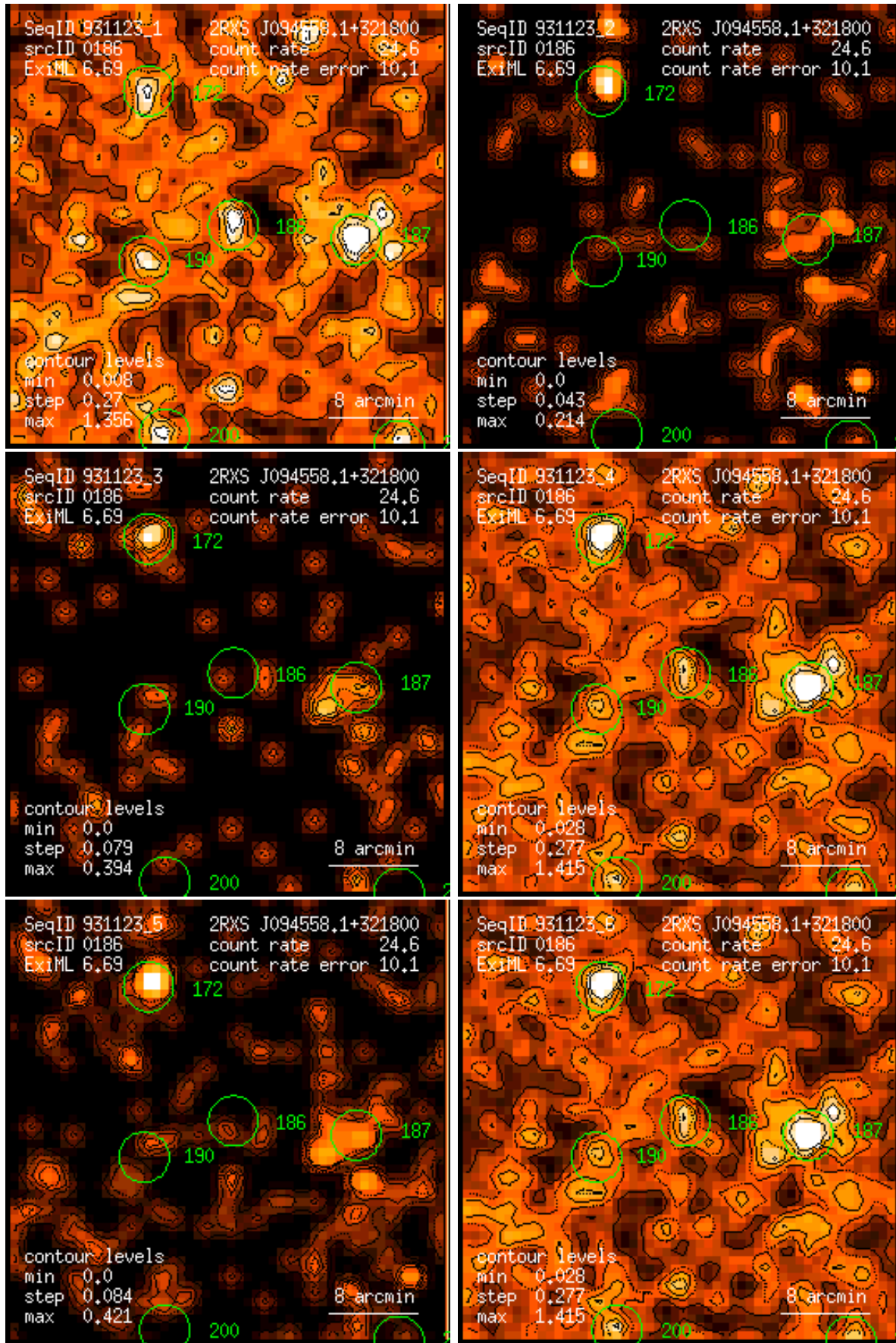
Figure 186: RASS 931123: detection 0186: band rate images, Gaussian filter: (1) PSPC channels 11 – 41, (2) 52 – 90, (3) 91 – 201, (4) 11 – 235, (5) 52 – 201, (6) 11 – 201. Broad band rates in counts/ks. Band rate contour levels in counts/ks/arcmin 2 .
