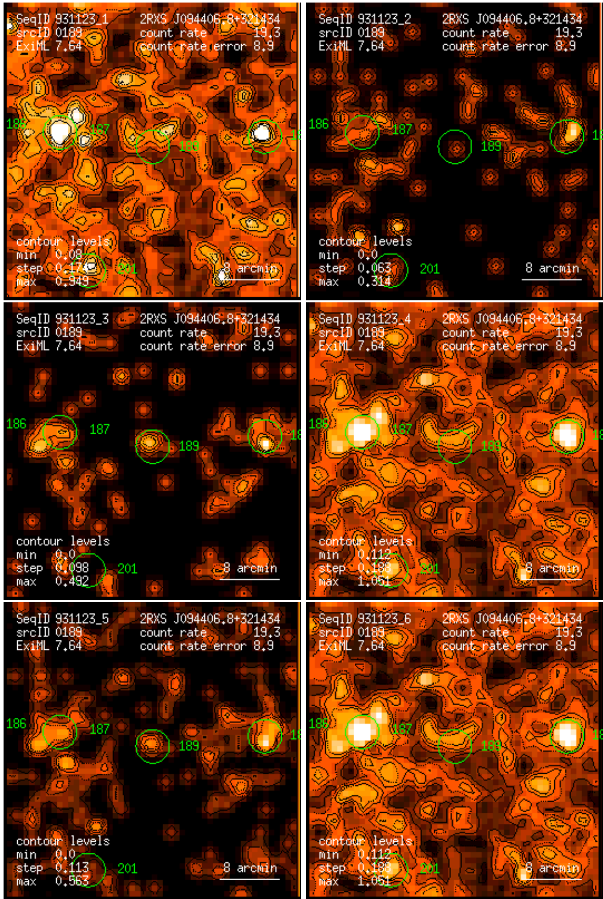
Figure 189: RASS 931123: detection 0189: band rate images, Gaussian filter: (1) PSPC channels 11 – 41, (2) 52 – 90, (3) 91 – 201, (4) 11 – 235, (5) 52 – 201, (6) 11 – 201. Broad band rates in counts/ks. Band rate contour levels in counts/ks/arcmin 2 .
