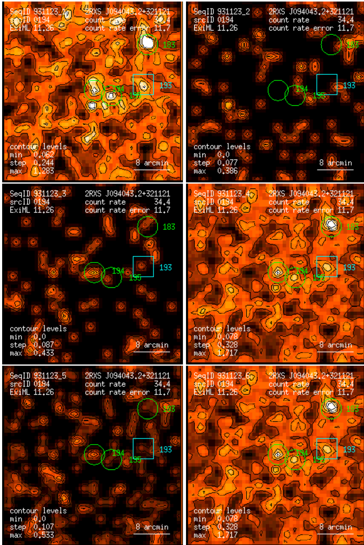
Figure 194: RASS 931123: detection 0194: band rate images, Gaussian filter: (1) PSPC channels 11 – 41, (2) 52 – 90, (3) 91 – 201, (4) 11 – 235, (5) 52 – 201, (6) 11 – 201. Broad band rates in counts/ks. Band rate contour levels in counts/ks/arcmin 2 .
