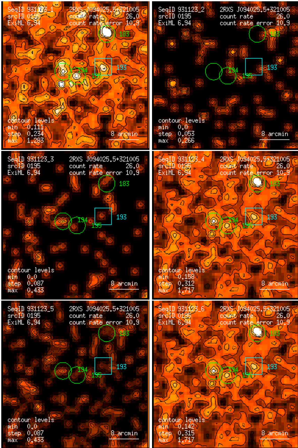
Figure 195: RASS 931123: detection 0195: band rate images, Gaussian filter: (1) PSPC channels 11 – 41, (2) 52 – 90, (3) 91 – 201, (4) 11 – 235, (5) 52 – 201, (6) 11 – 201. Broad band rates in counts/ks. Band rate contour levels in counts/ks/arcmin 2 .
