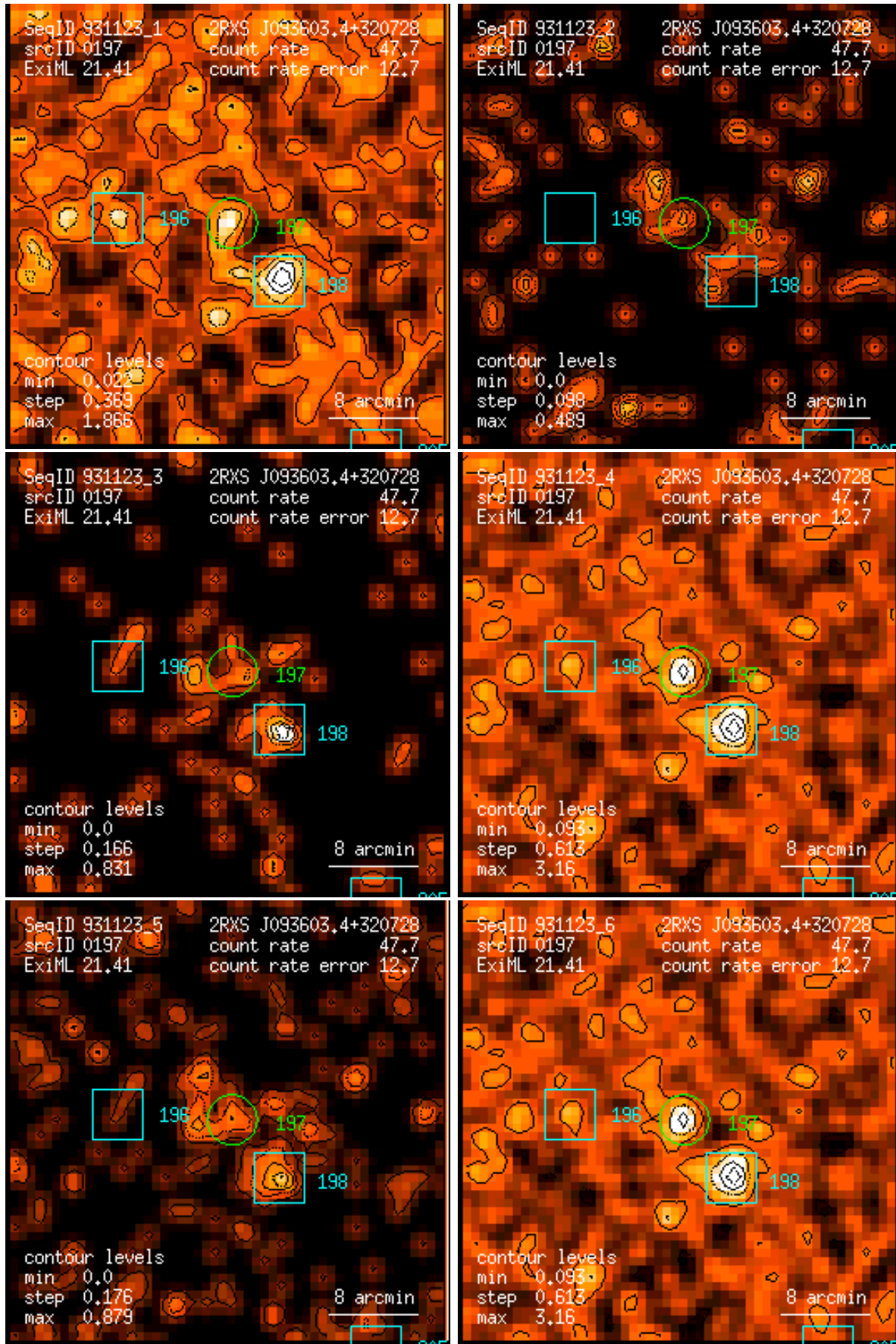
Figure 197: RASS 931123: detection 0197: band rate images, Gaussian filter: (1) PSPC channels 11 – 41, (2) 52 – 90, (3) 91 – 201, (4) 11 – 235, (5) 52 – 201, (6) 11 – 201. Broad band rates in counts/ks. Band rate contour levels in counts/ks/arcmin 2 .
