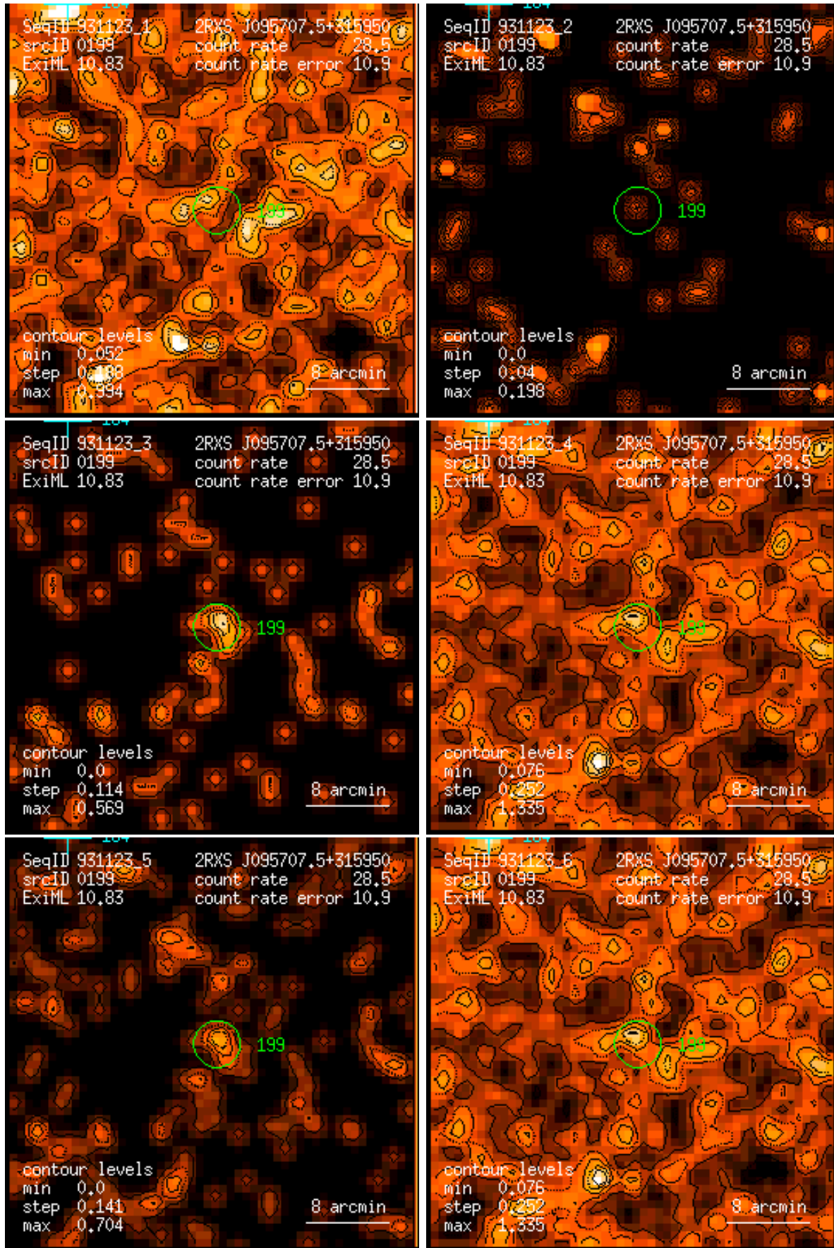
Figure 199: RASS 931123: detection 0199: band rate images, Gaussian filter: (1) PSPC channels 11 – 41, (2) 52 – 90, (3) 91 – 201, (4) 11 – 235, (5) 52 – 201, (6) 11 – 201. Broad band rates in counts/ks. Band rate contour levels in counts/ks/arcmin 2 .
