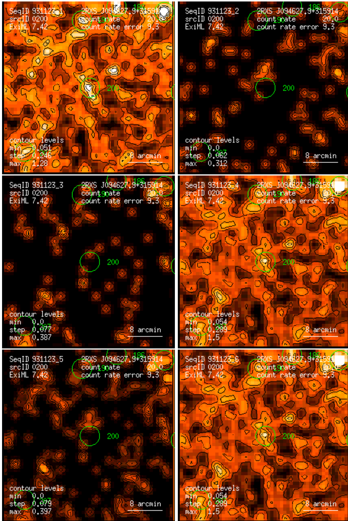
Figure 200: RASS 931123: detection 0200: band rate images, Gaussian filter: (1) PSPC channels 11 – 41, (2) 52 – 90, (3) 91 – 201, (4) 11 – 235, (5) 52 – 201, (6) 11 – 201. Broad band rates in counts/ks. Band rate contour levels in counts/ks/arcmin 2 .
