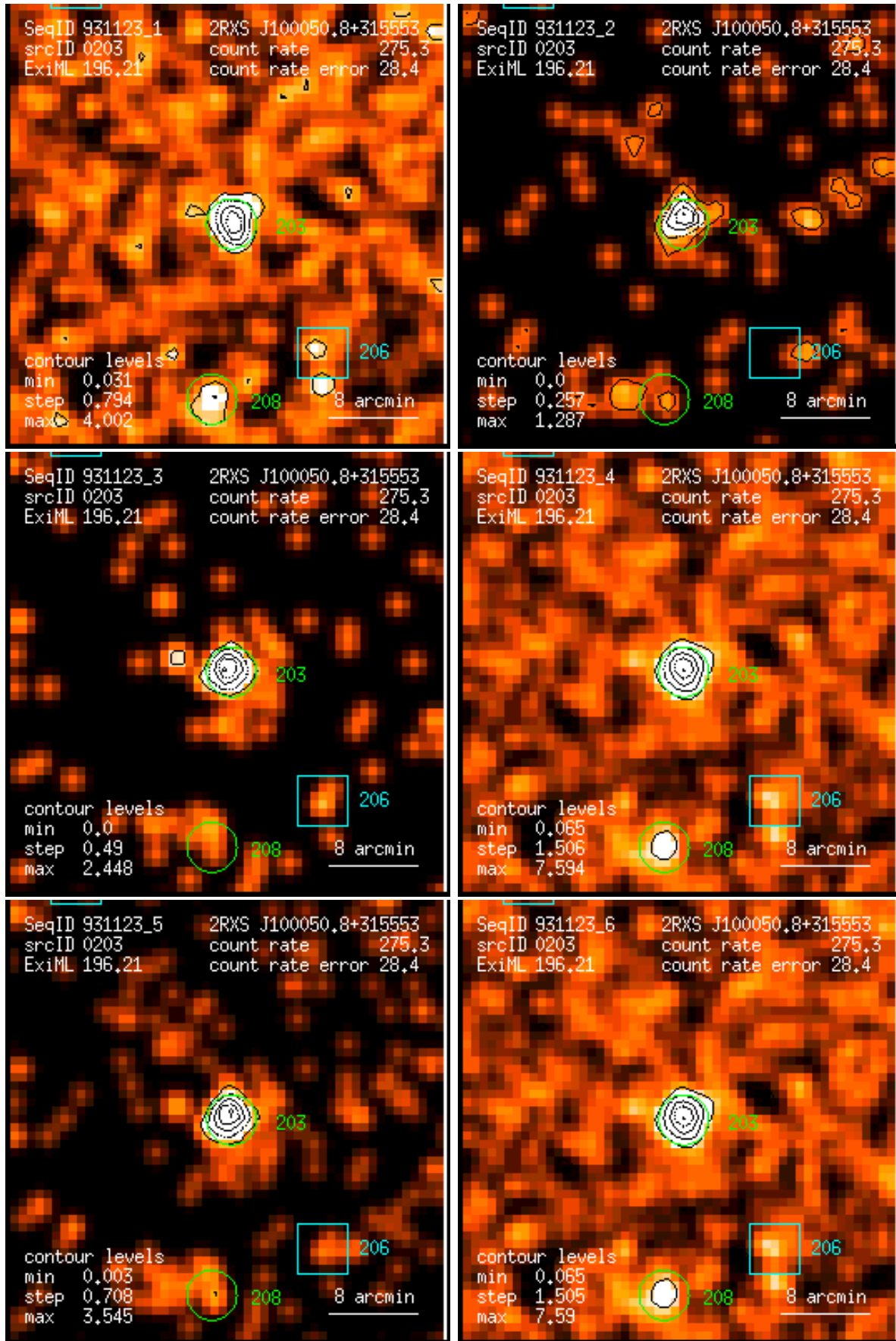
Figure 203: RASS 931123: detection 0203: band rate images, Gaussian filter: (1) PSPC channels 11 – 41, (2) 52 – 90, (3) 91 – 201, (4) 11 – 235, (5) 52 – 201, (6) 11 – 201. Broad band rates in counts/ks. Band rate contour levels in counts/ks/arcmin 2 .
