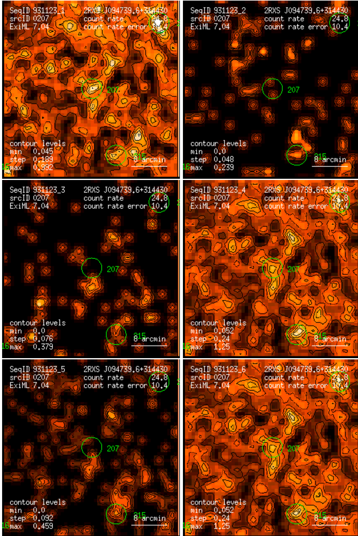
Figure 207: RASS 931123: detection 0207: band rate images, Gaussian filter: (1) PSPC channels 11 – 41, (2) 52 – 90, (3) 91 – 201, (4) 11 – 235, (5) 52 – 201, (6) 11 – 201. Broad band rates in counts/ks. Band rate contour levels in counts/ks/arcmin 2 .
