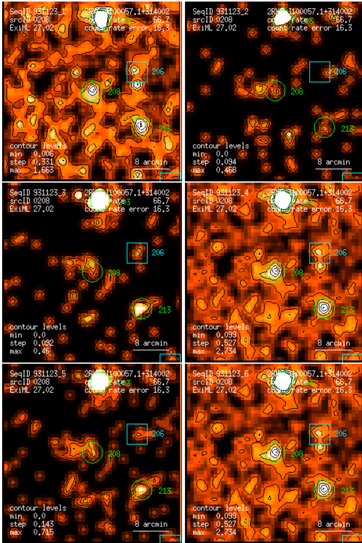
Figure 208: RASS 931123: detection 0208: band rate images, Gaussian filter: (1) PSPC channels 11 – 41, (2) 52 – 90, (3) 91 – 201, (4) 11 – 235, (5) 52 – 201, (6) 11 – 201. Broad band rates in counts/ks. Band rate contour levels in counts/ks/arcmin 2 .
