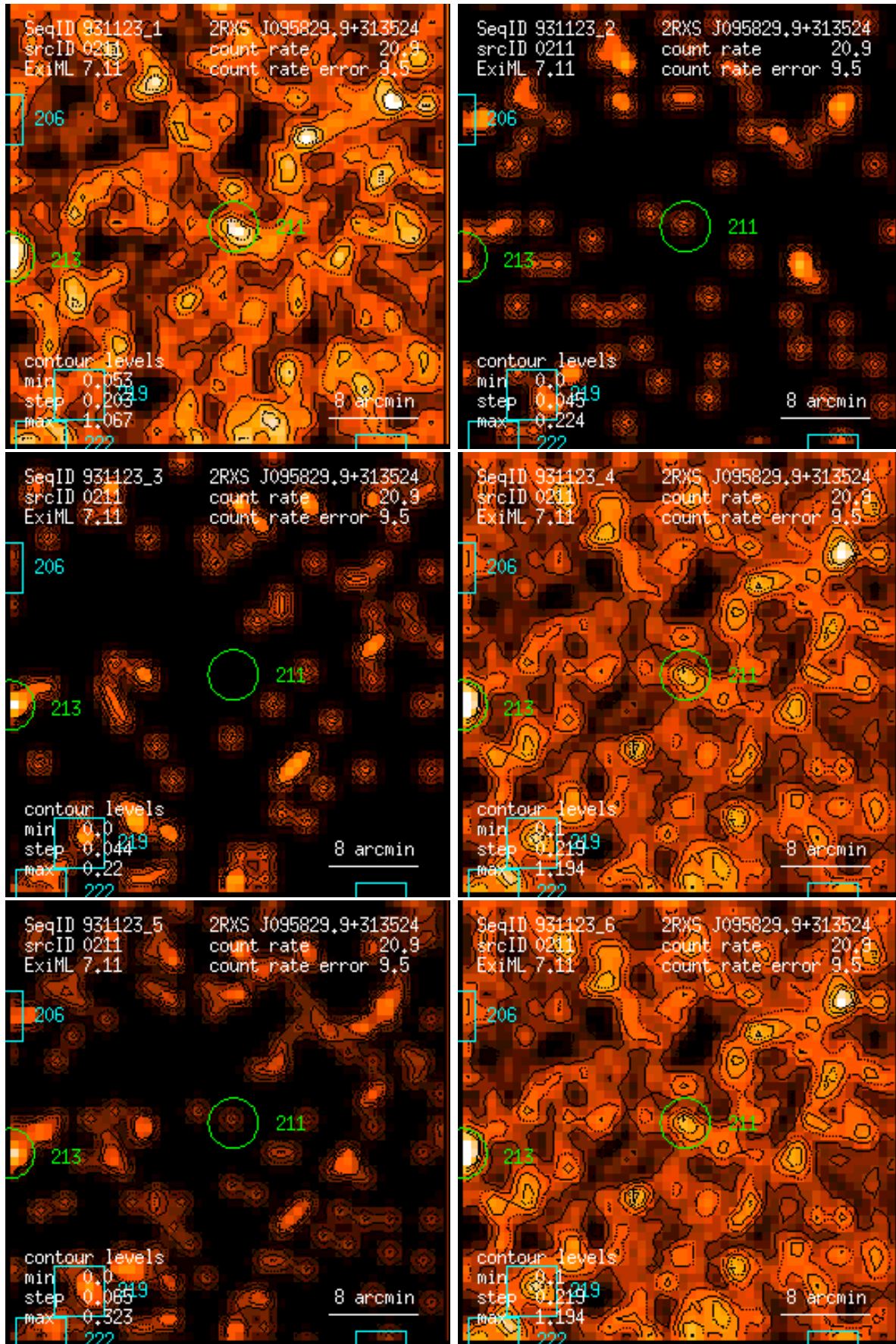
Figure 211: RASS 931123: detection 0211: band rate images, Gaussian filter: (1) PSPC channels 11 – 41, (2) 52 – 90, (3) 91 – 201, (4) 11 – 235, (5) 52 – 201, (6) 11 – 201. Broad band rates in counts/ks. Band rate contour levels in counts/ks/arcmin 2 .
