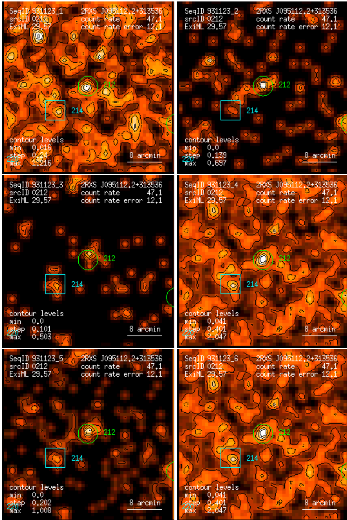
Figure 212: RASS 931123: detection 0212: band rate images, Gaussian filter: (1) PSPC channels 11 – 41, (2) 52 – 90, (3) 91 – 201, (4) 11 – 235, (5) 52 – 201, (6) 11 – 201. Broad band rates in counts/ks. Band rate contour levels in counts/ks/arcmin 2 .
