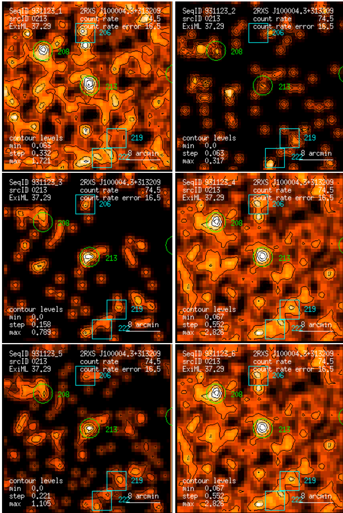
Figure 213: RASS 931123: detection 0213: band rate images, Gaussian filter: (1) PSPC channels 11 – 41, (2) 52 – 90, (3) 91 – 201, (4) 11 – 235, (5) 52 – 201, (6) 11 – 201. Broad band rates in counts/ks. Band rate contour levels in counts/ks/arcmin 2 .
