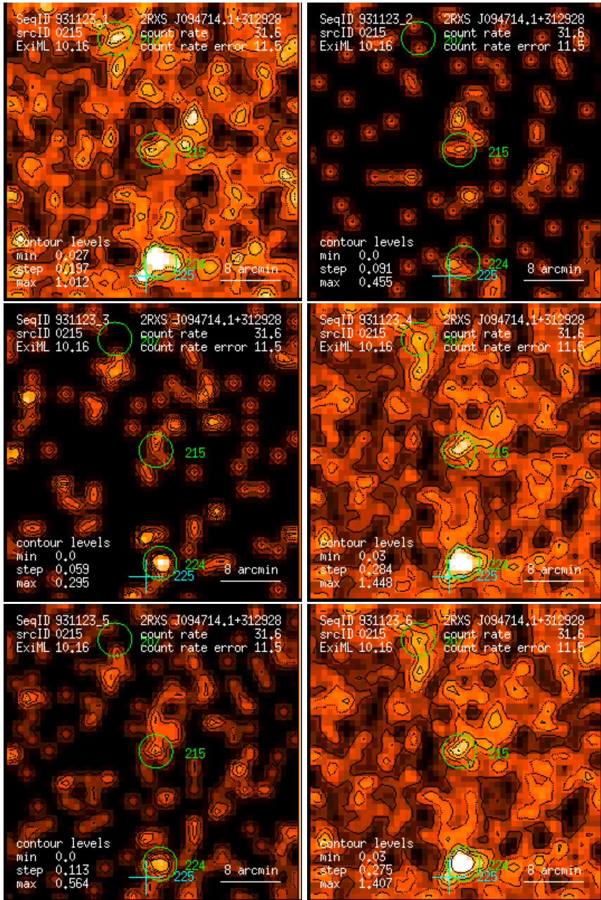
Figure 215: RASS 931123: detection 0215: band rate images, Gaussian filter: (1) PSPC channels 11 – 41, (2) 52 – 90, (3) 91 – 201, (4) 11 – 235, (5) 52 – 201, (6) 11 – 201. Broad band rates in counts/ks. Band rate contour levels in counts/ks/arcmin 2 .
