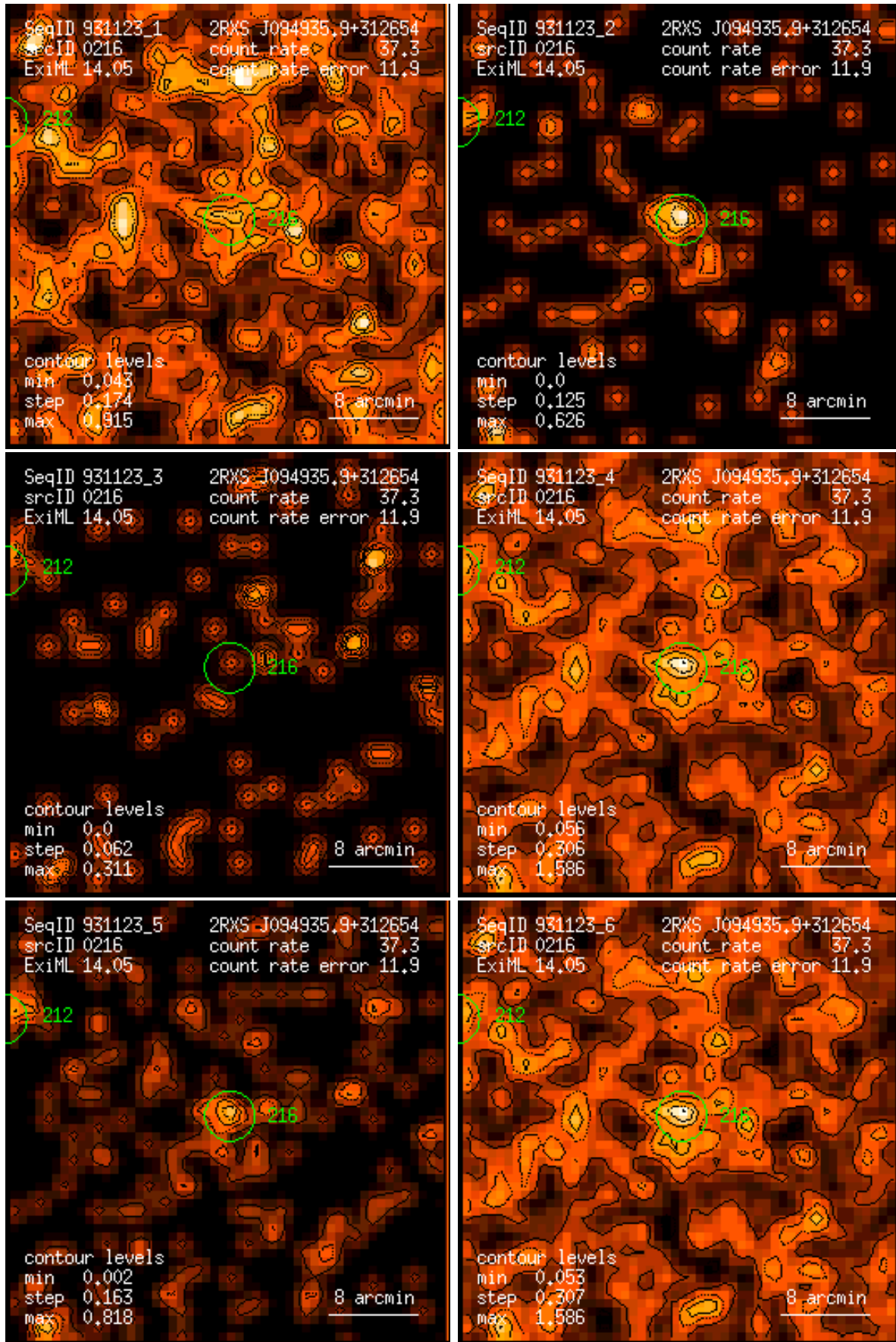
Figure 216: RASS 931123: detection 0216: band rate images, Gaussian filter: (1) PSPC channels 11 – 41, (2) 52 – 90, (3) 91 – 201, (4) 11 – 235, (5) 52 – 201, (6) 11 – 201. Broad band rates in counts/ks. Band rate contour levels in counts/ks/arcmin 2 .
