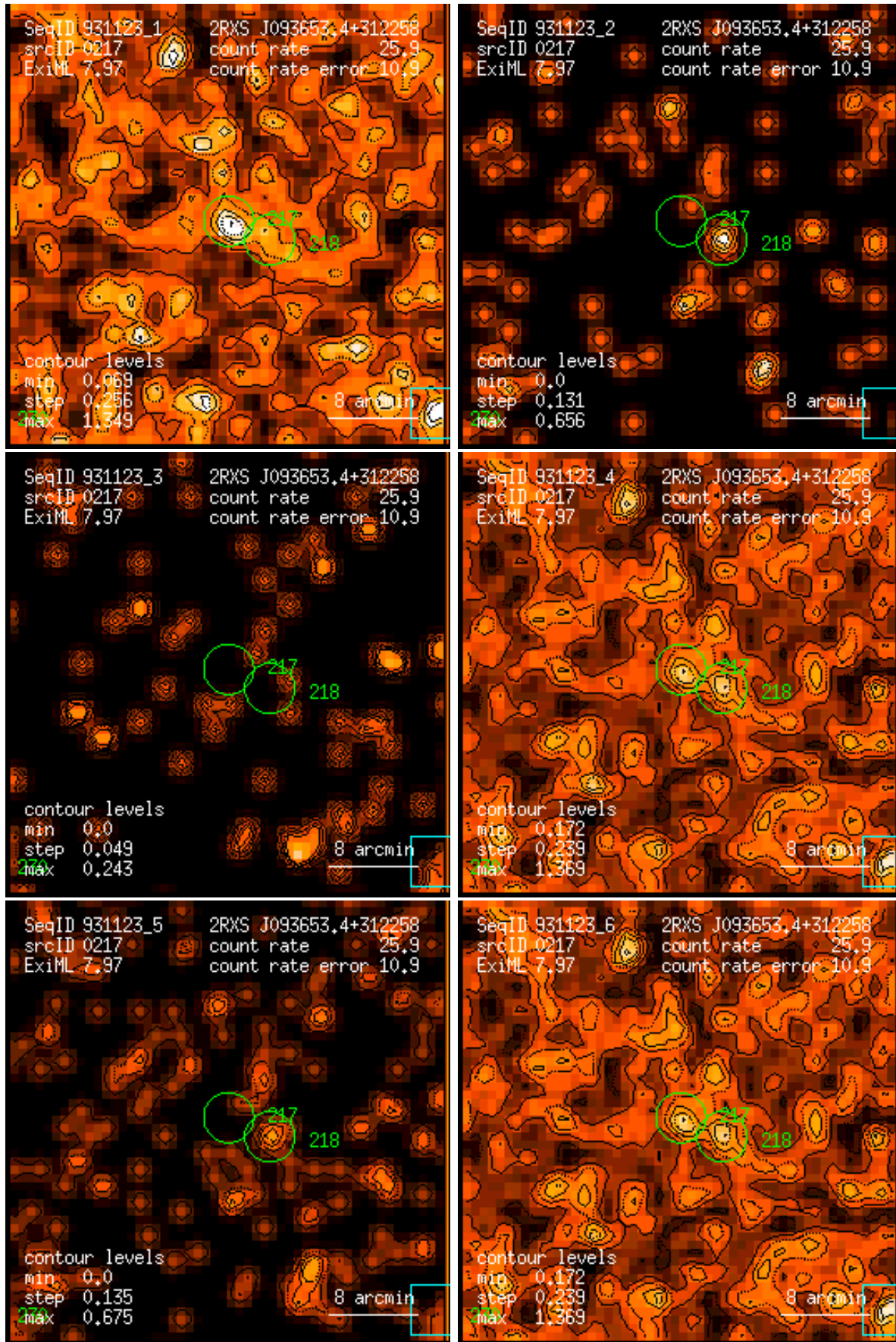
Figure 217: RASS 931123: detection 0217: band rate images, Gaussian filter: (1) PSPC channels 11 – 41, (2) 52 – 90, (3) 91 – 201, (4) 11 – 235, (5) 52 – 201, (6) 11 – 201. Broad band rates in counts/ks. Band rate contour levels in counts/ks/arcmin 2 .
