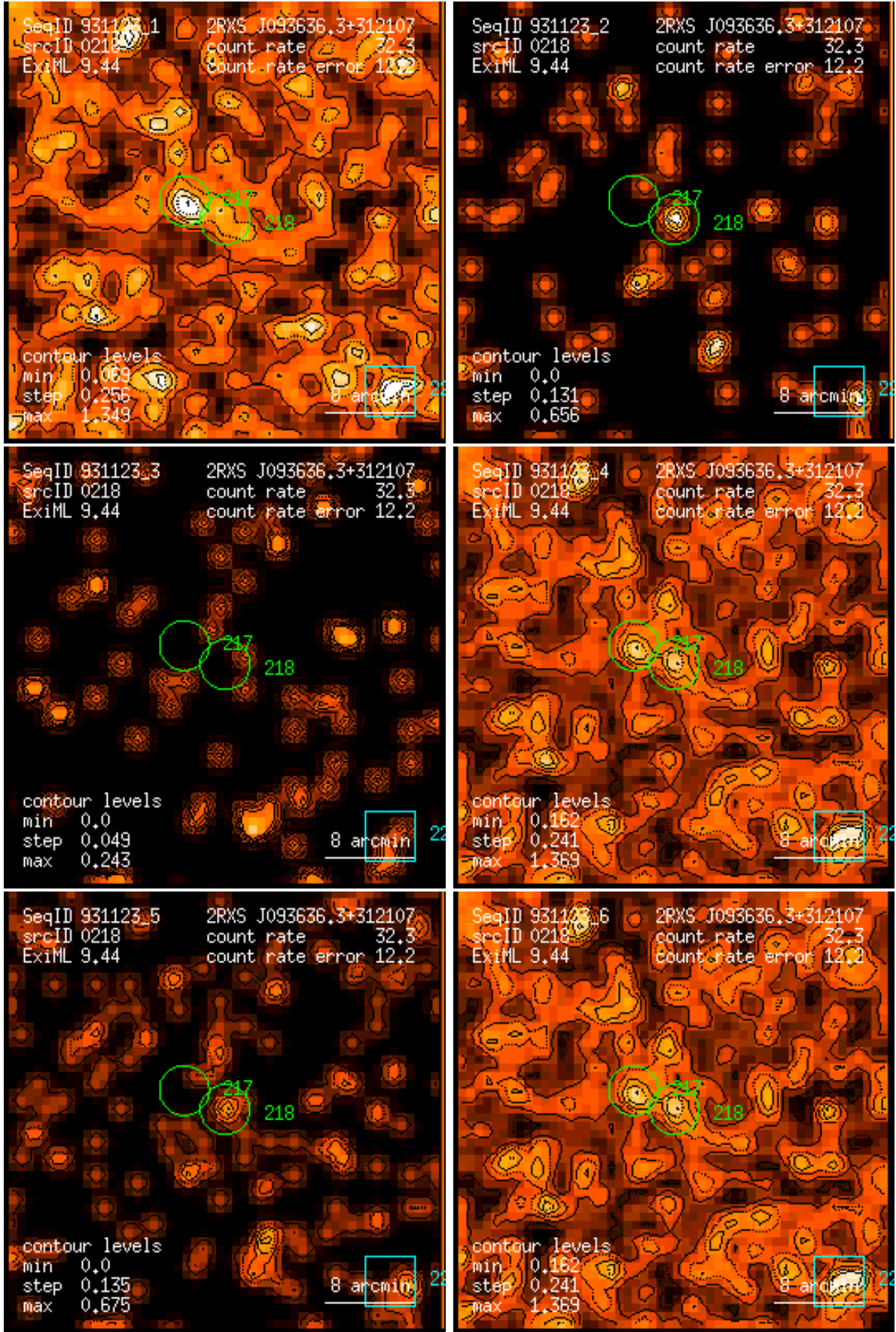
Figure 218: RASS 931123: detection 0218: band rate images, Gaussian filter: (1) PSPC channels 11 – 41, (2) 52 – 90, (3) 91 – 201, (4) 11 – 235, (5) 52 – 201, (6) 11 – 201. Broad band rates in counts/ks. Band rate contour levels in counts/ks/arcmin 2 .
