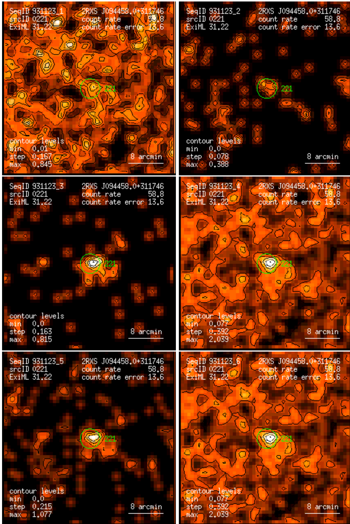
Figure 221: RASS 931123: detection 0221: band rate images, Gaussian filter: (1) PSPC channels 11 – 41, (2) 52 – 90, (3) 91 – 201, (4) 11 – 235, (5) 52 – 201, (6) 11 – 201. Broad band rates in counts/ks. Band rate contour levels in counts/ks/arcmin 2 .
