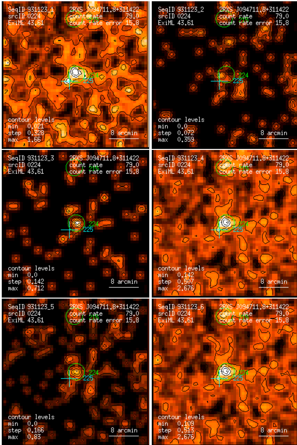
Figure 224: RASS 931123: detection 0224: band rate images, Gaussian filter: (1) PSPC channels 11 – 41, (2) 52 – 90, (3) 91 – 201, (4) 11 – 235, (5) 52 – 201, (6) 11 – 201. Broad band rates in counts/ks. Band rate contour levels in counts/ks/arcmin 2 .
