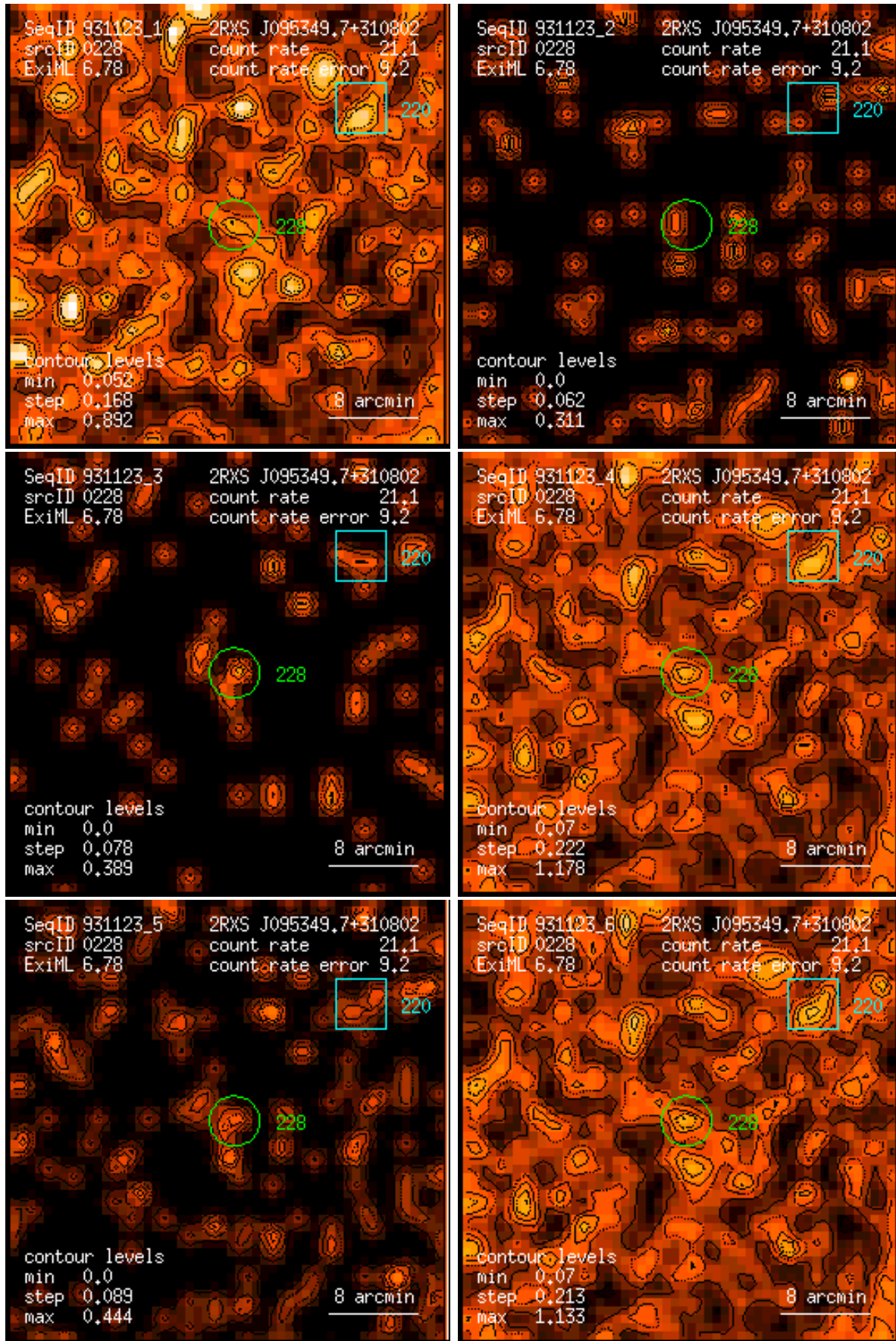
Figure 228: RASS 931123: detection 0228: band rate images, Gaussian filter: (1) PSPC channels 11 – 41, (2) 52 – 90, (3) 91 – 201, (4) 11 – 235, (5) 52 – 201, (6) 11 – 201. Broad band rates in counts/ks. Band rate contour levels in counts/ks/arcmin 2 .
