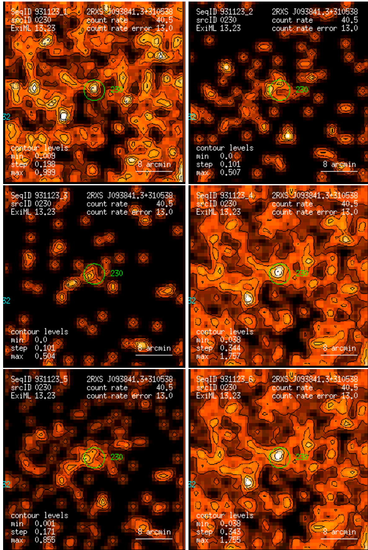
Figure 230: RASS 931123: detection 0230: band rate images, Gaussian filter: (1) PSPC channels 11 – 41, (2) 52 – 90, (3) 91 – 201, (4) 11 – 235, (5) 52 – 201, (6) 11 – 201. Broad band rates in counts/ks. Band rate contour levels in counts/ks/arcmin 2 .
