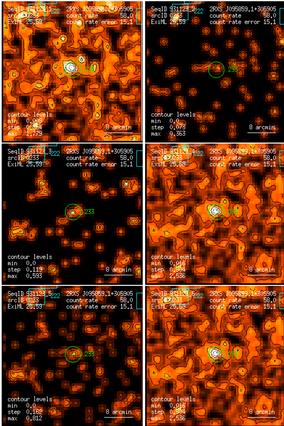
Figure 233: RASS 931123: detection 0233: band rate images, Gaussian filter: (1) PSPC channels 11 – 41, (2) 52 – 90, (3) 91 – 201, (4) 11 – 235, (5) 52 – 201, (6) 11 – 201. Broad band rates in counts/ks. Band rate contour levels in counts/ks/arcmin 2 .
