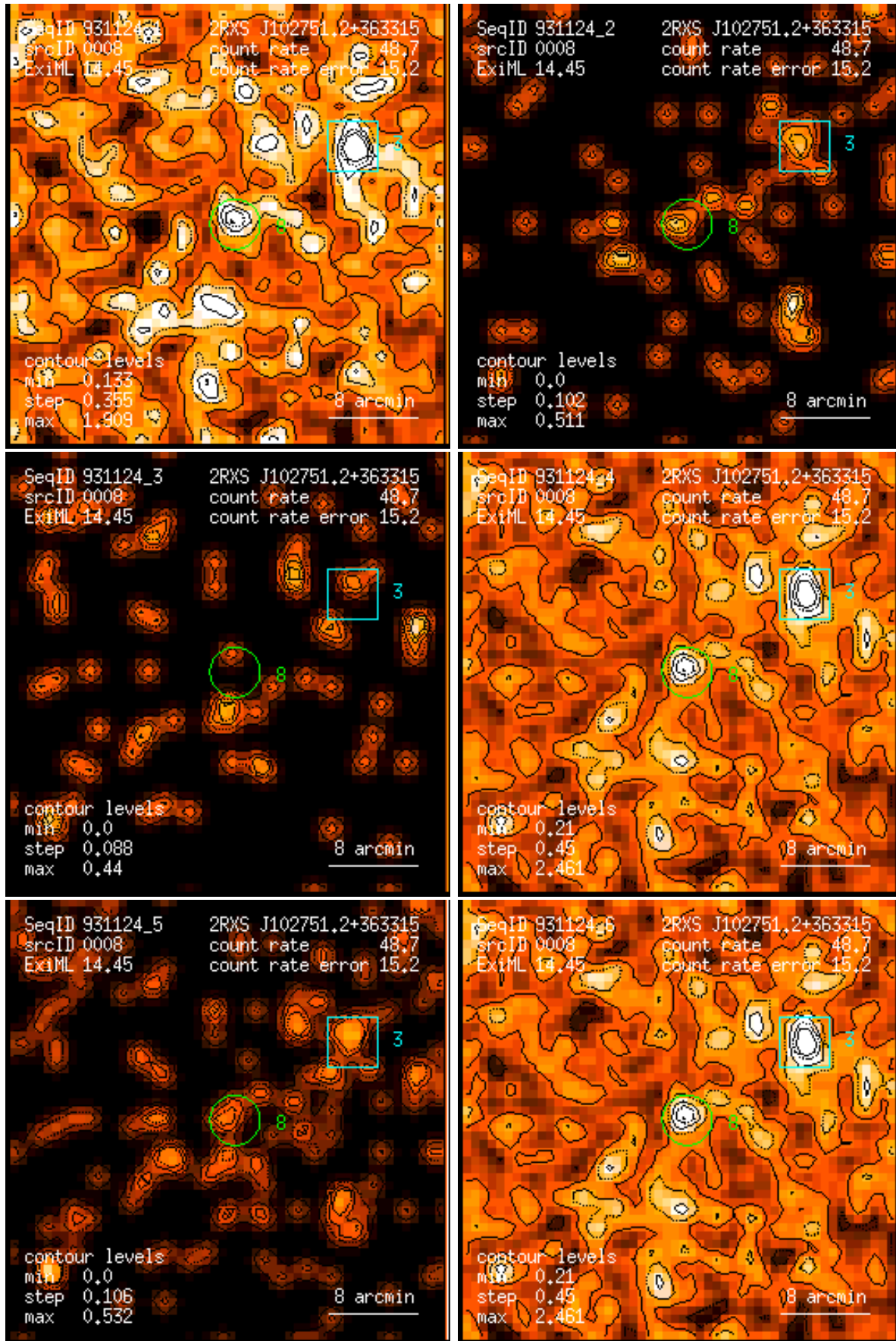
Figure 8: RASS 931124: detection 0008: band rate images, Gaussian filter: (1) PSPC channels 11 – 41, (2) 52 – 90, (3) 91 – 201, (4) 11 – 235, (5) 52 – 201, (6) 11 – 201. Broad band rates in counts/ks. Band rate contour levels in counts/ks/arcmin 2 .
