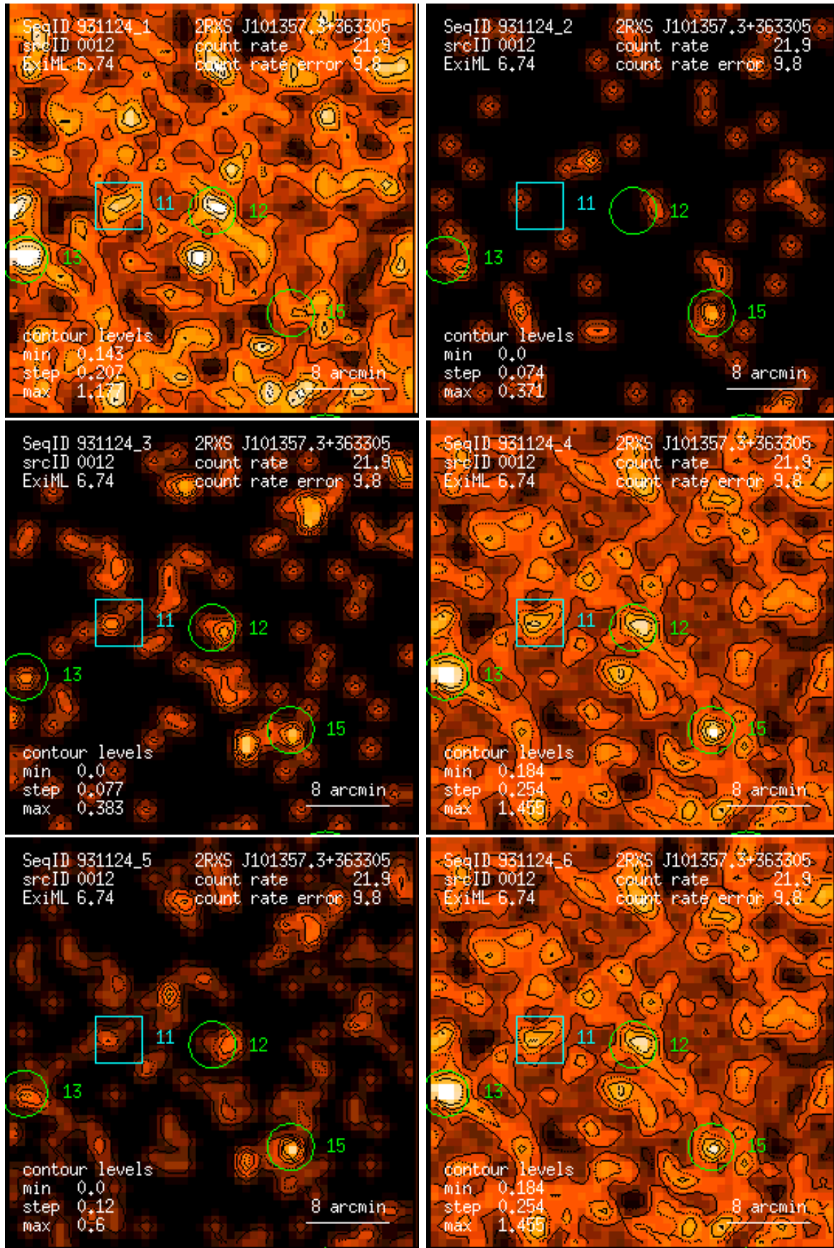
Figure 12: RASS 931124: detection 0012: band rate images, Gaussian filter: (1) PSPC channels 11 – 41, (2) 52 – 90, (3) 91 – 201, (4) 11 – 235, (5) 52 – 201, (6) 11 – 201. Broad band rates in counts/ks. Band rate contour levels in counts/ks/arcmin 2 .
