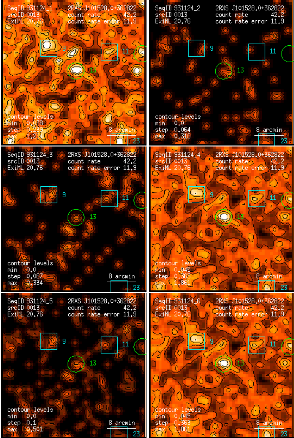
Figure 13: RASS 931124: detection 0013: band rate images, Gaussian filter: (1) PSPC channels 11 – 41, (2) 52 – 90, (3) 91 – 201, (4) 11 – 235, (5) 52 – 201, (6) 11 – 201. Broad band rates in counts/ks. Band rate contour levels in counts/ks/arcmin 2 .
