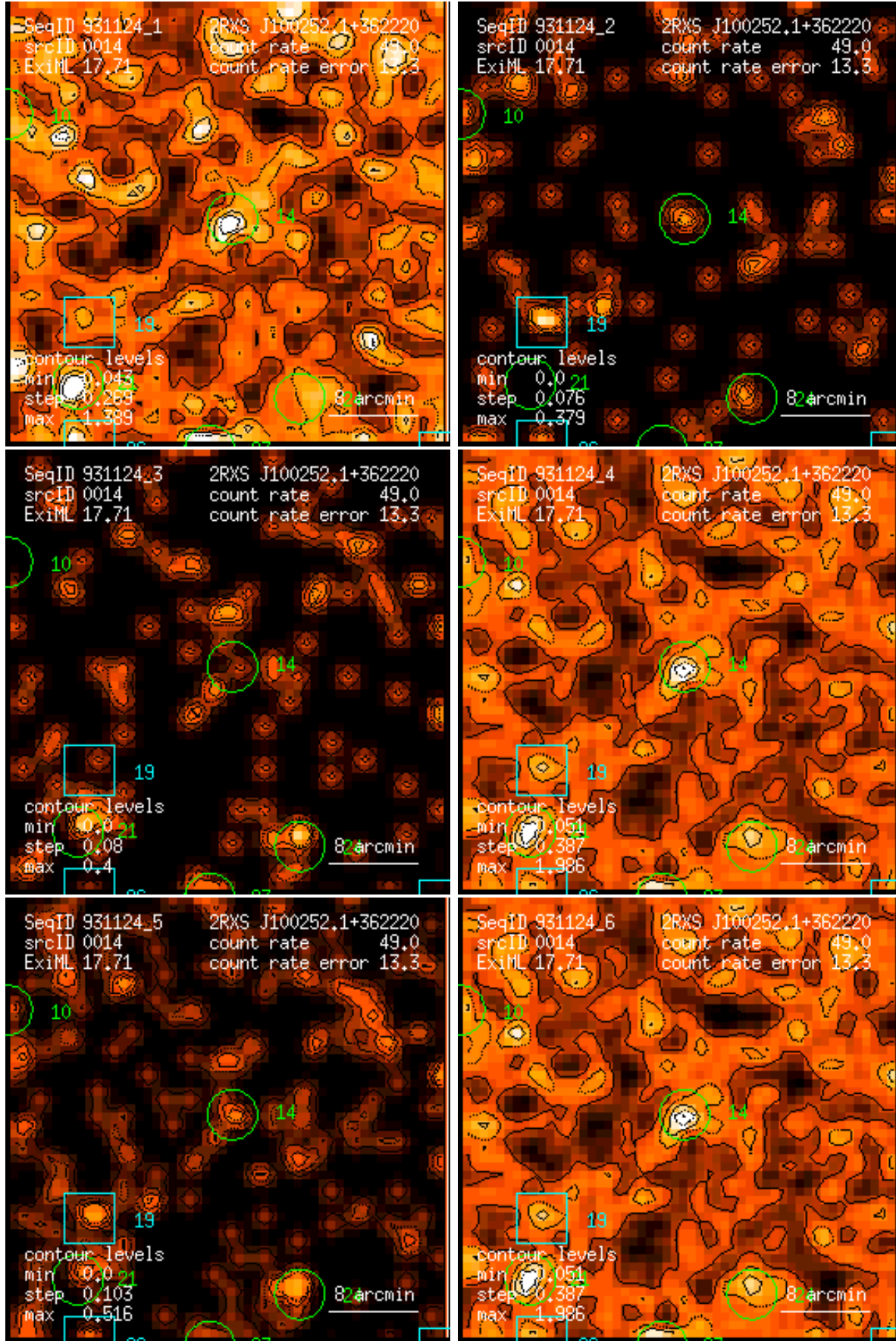
Figure 14: RASS 931124: detection 0014: band rate images, Gaussian filter: (1) PSPC channels 11 – 41, (2) 52 – 90, (3) 91 – 201, (4) 11 – 235, (5) 52 – 201, (6) 11 – 201. Broad band rates in counts/ks. Band rate contour levels in counts/ks/arcmin 2 .
