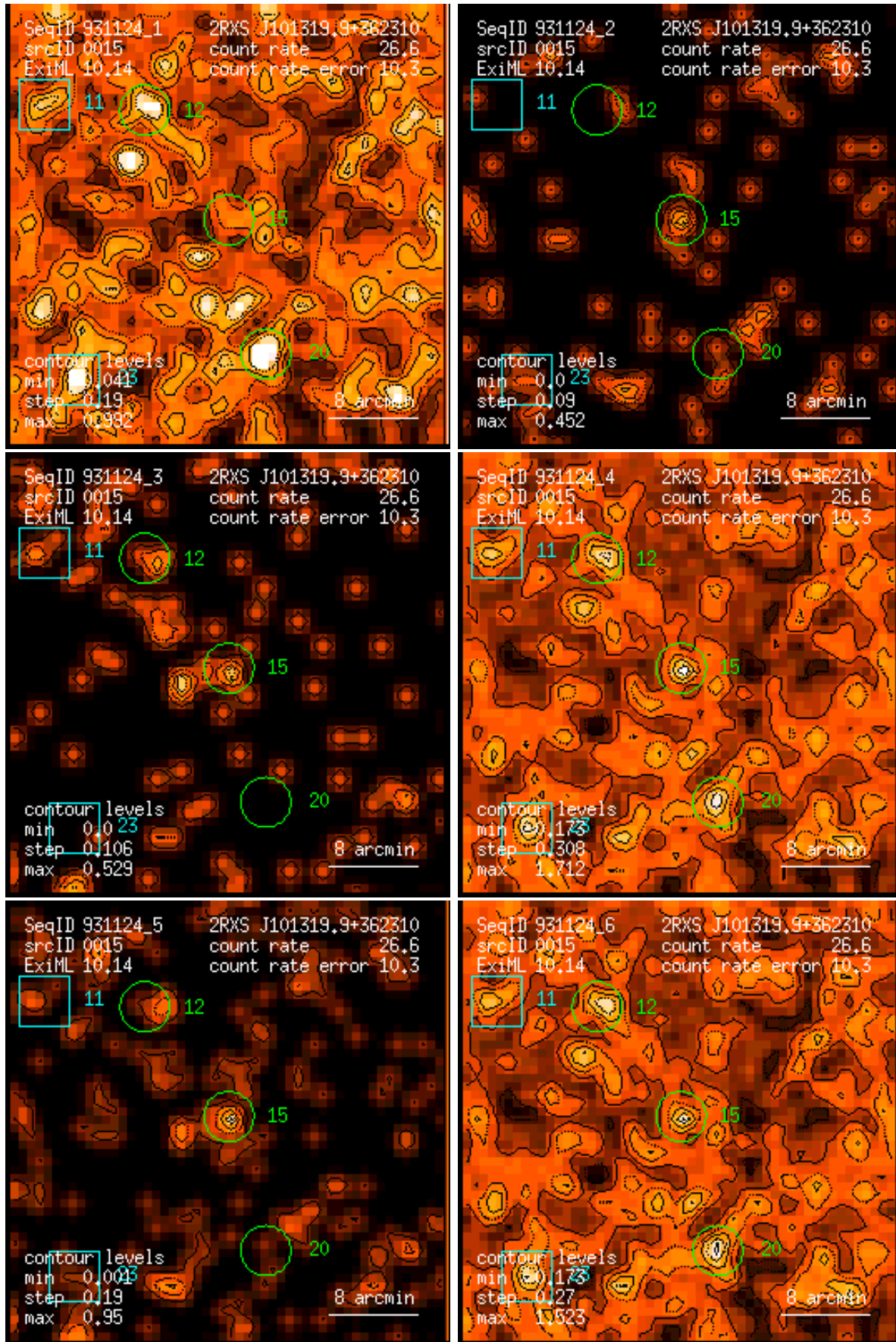
Figure 15: RASS 931124: detection 0015: band rate images, Gaussian filter: (1) PSPC channels 11 – 41, (2) 52 – 90, (3) 91 – 201, (4) 11 – 235, (5) 52 – 201, (6) 11 – 201. Broad band rates in counts/ks. Band rate contour levels in counts/ks/arcmin 2 .
