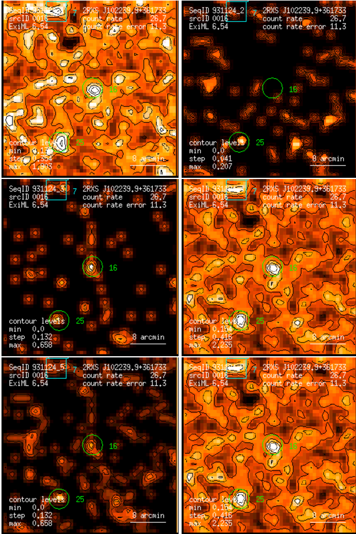
Figure 16: RASS 931124: detection 0016: band rate images, Gaussian filter: (1) PSPC channels 11 – 41, (2) 52 – 90, (3) 91 – 201, (4) 11 – 235, (5) 52 – 201, (6) 11 – 201. Broad band rates in counts/ks. Band rate contour levels in counts/ks/arcmin 2 .
