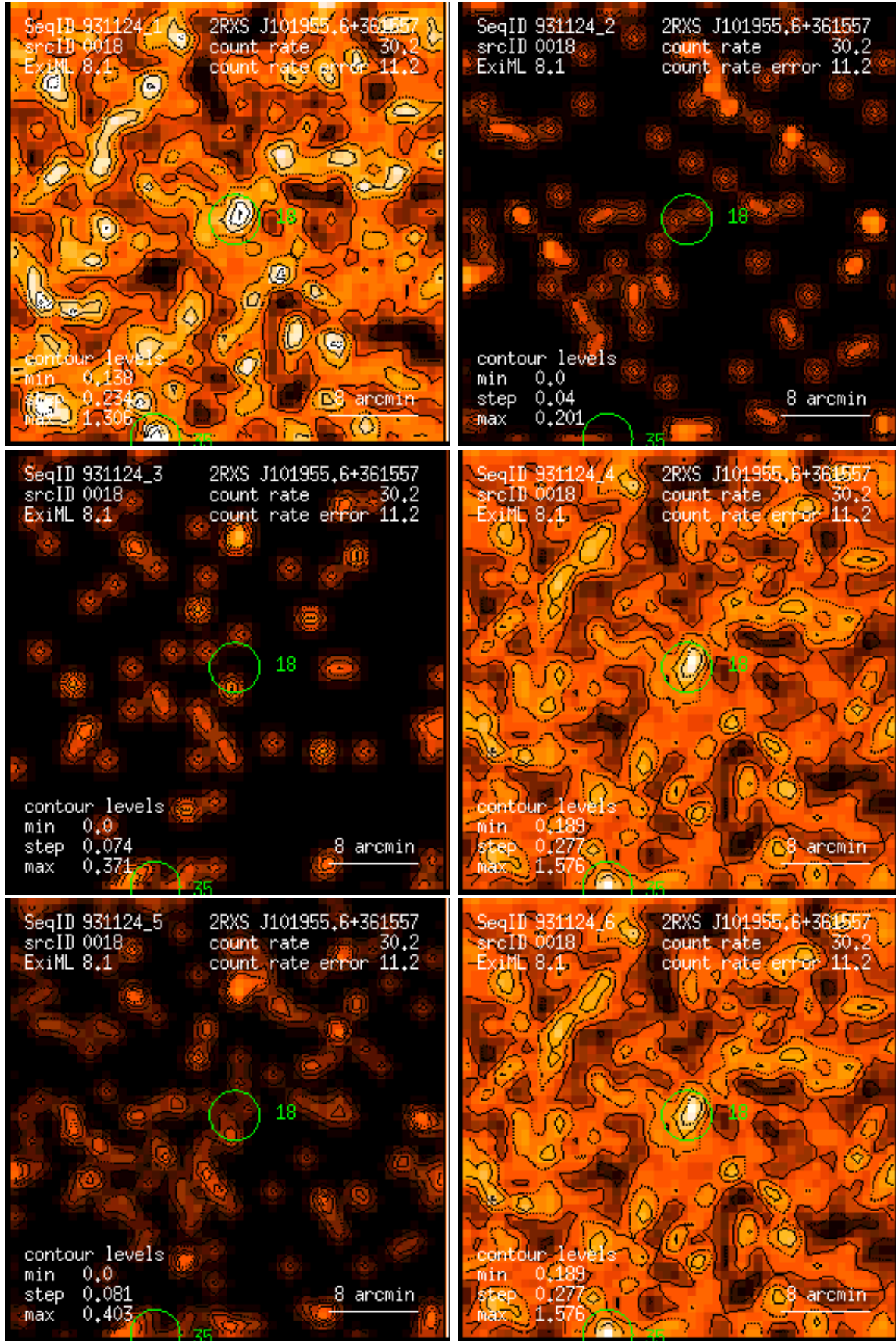
Figure 18: RASS 931124: detection 0018: band rate images, Gaussian filter: (1) PSPC channels 11 – 41, (2) 52 – 90, (3) 91 – 201, (4) 11 – 235, (5) 52 – 201, (6) 11 – 201. Broad band rates in counts/ks. Band rate contour levels in counts/ks/arcmin 2 .
