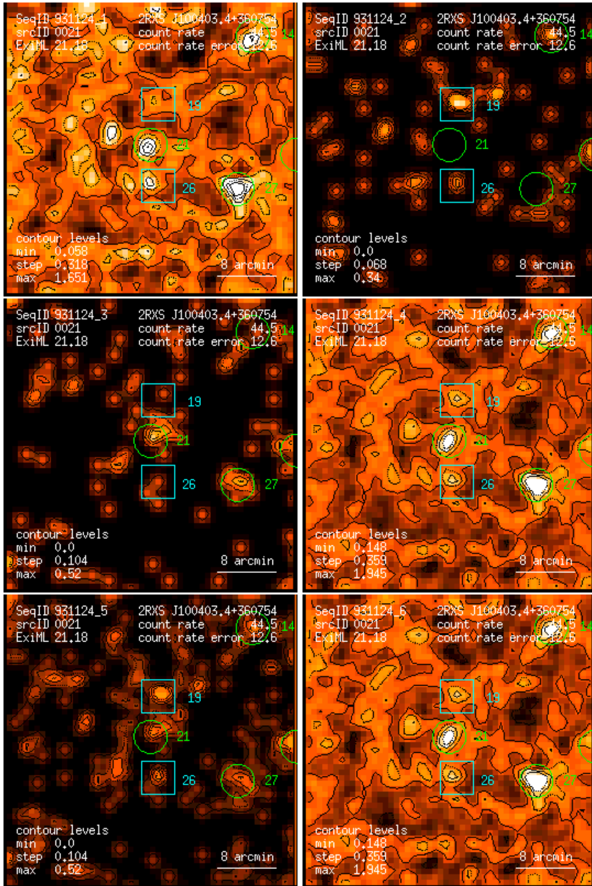
Figure 21: RASS 931124: detection 0021: band rate images, Gaussian filter: (1) PSPC channels 11 – 41, (2) 52 – 90, (3) 91 – 201, (4) 11 – 235, (5) 52 – 201, (6) 11 – 201. Broad band rates in counts/ks. Band rate contour levels in counts/ks/arcmin 2 .
