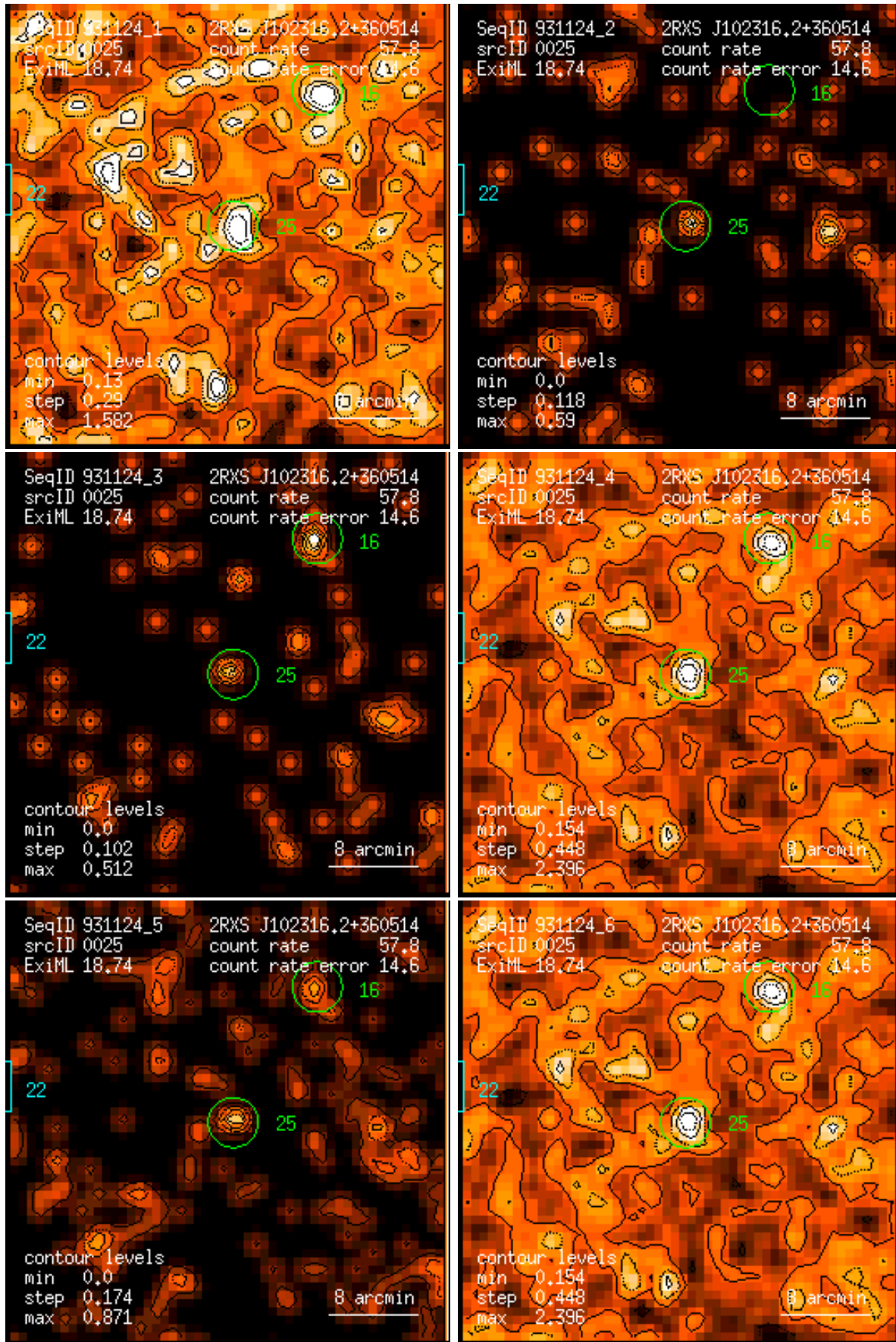
Figure 25: RASS 931124: detection 0025: band rate images, Gaussian filter: (1) PSPC channels 11 – 41, (2) 52 – 90, (3) 91 – 201, (4) 11 – 235, (5) 52 – 201, (6) 11 – 201. Broad band rates in counts/ks. Band rate contour levels in counts/ks/arcmin 2 .
